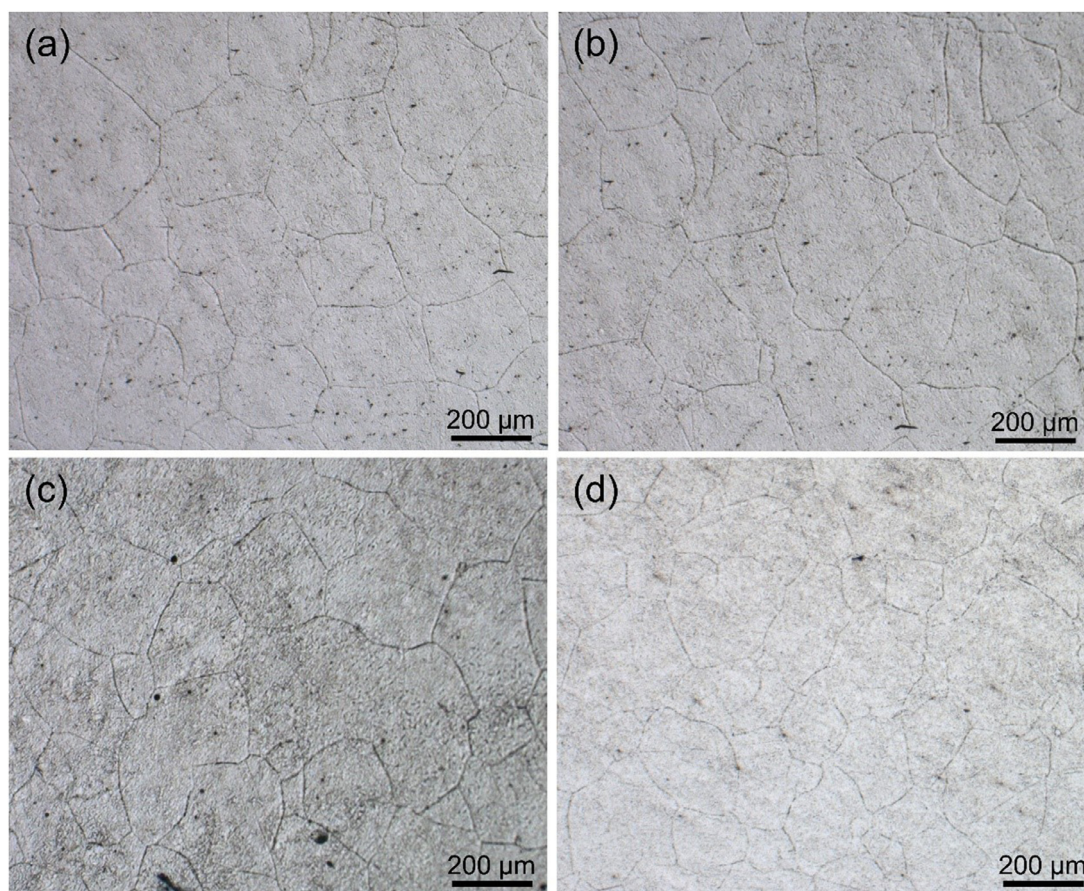
Fig. 3. Optical micrographs of the (a) sample A, (b) sample B1, (c) sample B4, (d) sample B6 etched to reveal the PAG.
