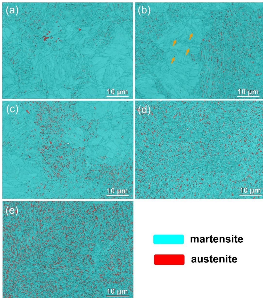
Fig. 5. BCE maps with the phases of samples with different numbers of CQT cycles from EBSD analysis: (a) sample B1, (b) sample B2, (c) sample B3, (d) sample B4, and (e) sample B6.
