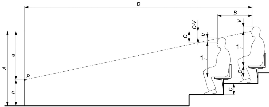
Fig. 5. The diagram of the riser calculation [5].
