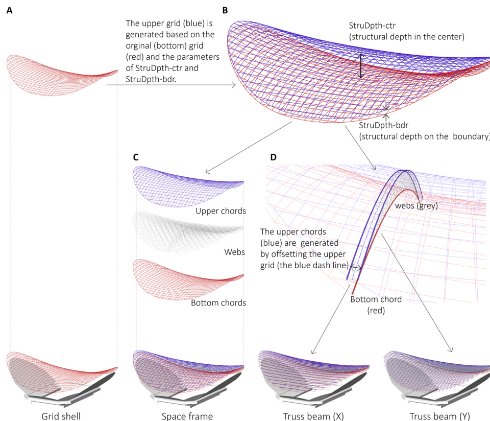
Fig. 6. The generation of the roof structure.
