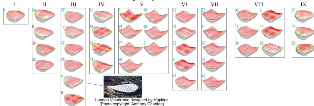
Fig. 12. Results of OPT.1 (solutions with grid-shell, space-frame, and truss-beam structures are labelled in green, blue, and red, respectively) (picture source [69]).
