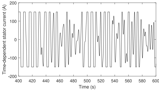
Fig. 4. The profile of the time-dependent stator current of the generator with a current limit, with H_t = 2.5 m, T_p = 7.5 s and B_{pto} = 60 kN s/m.
