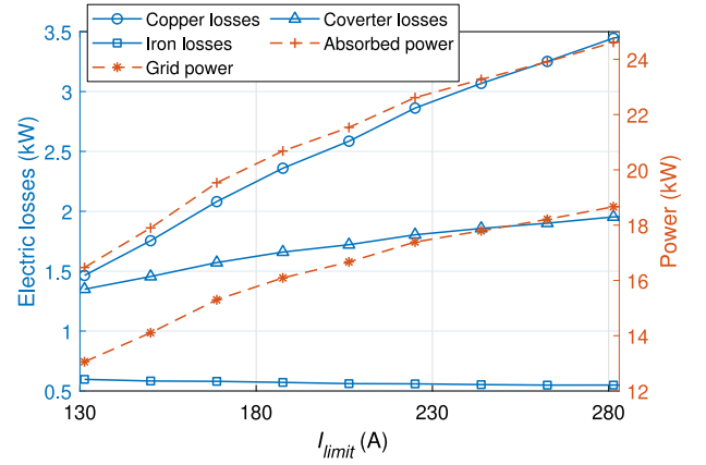
Fig. 14. The power and electric losses of the WEC with different current limits, and with T_p = 7.5 s and B_{pto} = 80 kN s/m. The results are generated by TD model.
