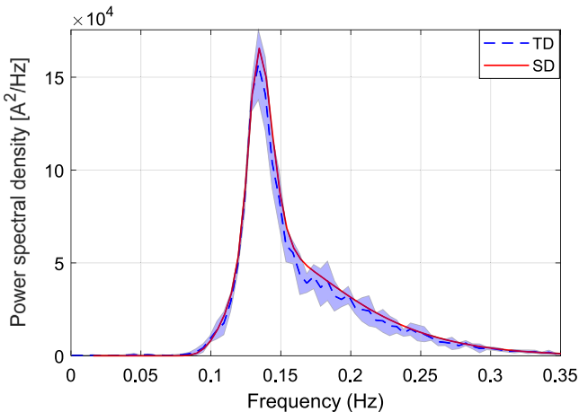
Fig. 13. The power spectral density of the stator current with a current limit of 150 A. ( B_{pto} = 80 kN s/m, H_s = 2.5 m and T_p = 7.5 s) The shaded area represents the standard deviation of the results of the TD model.
