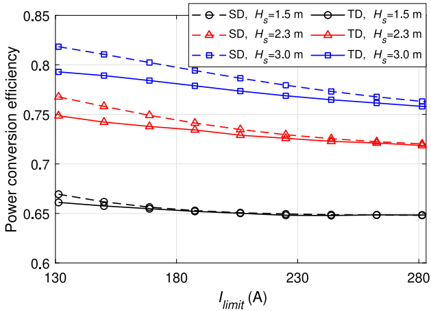
Fig. 12. The power conversion efficiency of the WEC with different current limits, and with T_p = 7.5 s and B_{pto} = 80 kN s/m.
