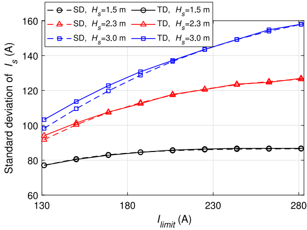
Fig. 11. The standard deviation of the stator current of the generator with different current limits, and with T_p = 7.5 s and B_{pto} = 80 kN s/m.
