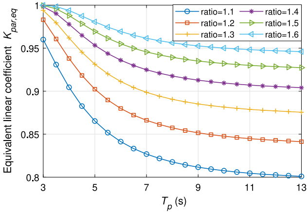
Fig. 9. The derived linear equivalent coefficient for the partial overlap effect K_{par,eq} with different translator lengths. The simulation is implemented in the case with H_s of 3.0 m and B_{pto} of 60 kN s/m. The “ratio” in the legend indicates the ratio between the translator length and stator length, and the stator length is considered constant as 2.3 m.
