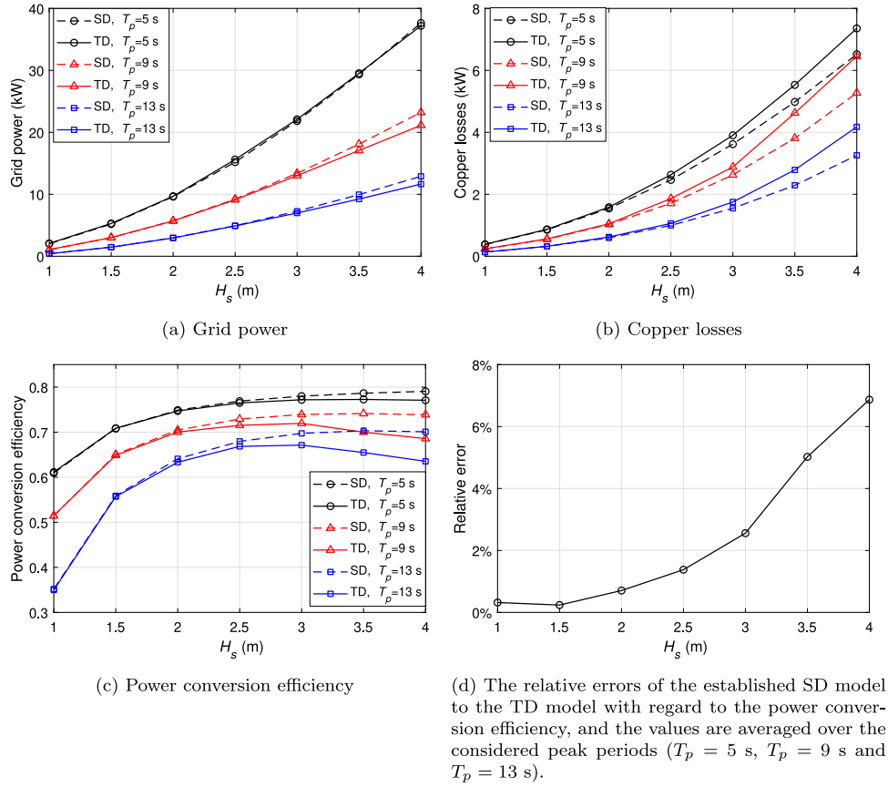
Fig. 8. Grid power, copper losses and power conversion efficiency of the WEC in different wave states and the relative errors of the SD model to the TD model. ( B_{pto} = 60 kN s/m).
