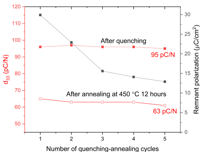
FIG. 11. Piezoelectric and ferroelectric properties after multiple quenching-annealing cycles. Symbol colors correspond to the label colors on the X and Y axes.
