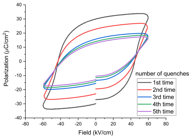
FIG. 10. P-E loops after multiple cycles of quenching from 700 °C in oil with subsequent 12 h annealing in air at 450 °C.
