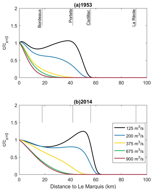
Figure 7. Evolution of tidally averaged c/c_{x0} at the surface of the GTR with river discharge for the years (a) 1953 and (b) 2014. GTR, Garonne Tidal River.
