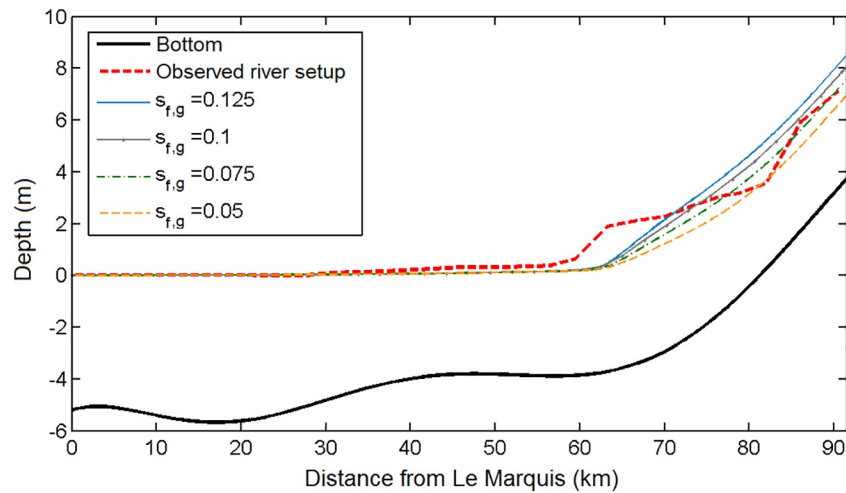
Figure 3. Comparison of observed and modeled river flow setups for different values of s_{f,g} .
