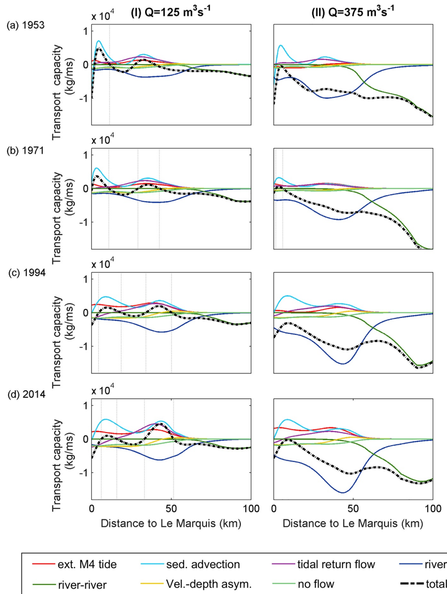
Figure 9. Contribution of the different physical mechanisms to the sediment-transport capacity per meter width (and integrated over depth). Negative values indicate export, while positive values indicate import. The total net transport of all term is plotted in black dashed line. Spring tide (tidal range of 3.75 m at the estuary mouth) and river discharges of (I) 125 \text{ m}^3/\text{s} and (II) 375 \text{ m}^3/\text{s} for (a) 1953, (b) 1971, (c) 1994, and (d) 2014.
