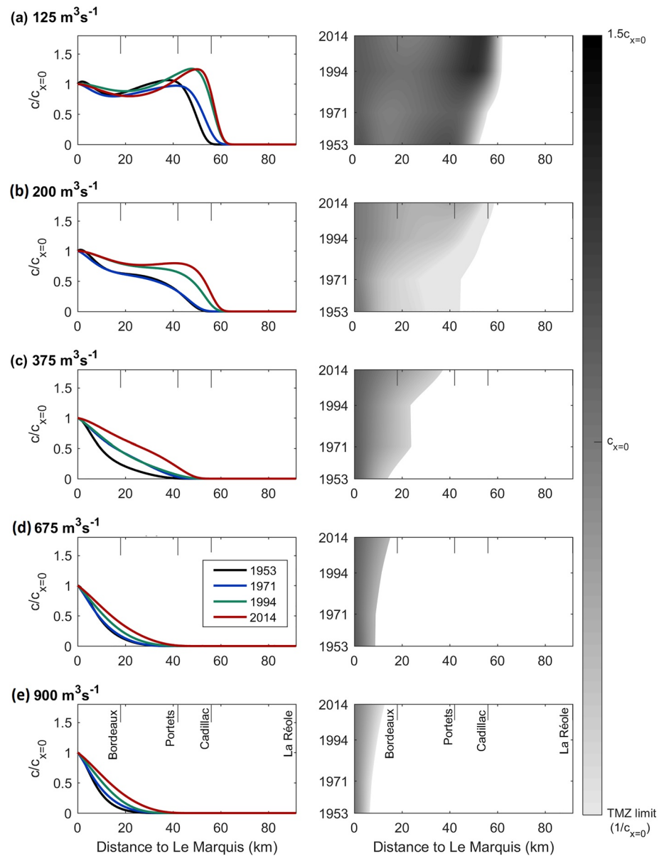
Figure 8. Multidecadal evolution of tidally averaged c/c_{x=0} at the surface of the GTR for five levels of river discharge: (a) 125 \text{ m}^3/\text{s} , (b) 200 \text{ m}^3/\text{s} , (c) 375 \text{ m}^3/\text{s} , (d) 675 \text{ m}^3/\text{s} , and (e) 900 \text{ m}^3/\text{s} . Right panels show the interpolation of data presented in left panels over time.
