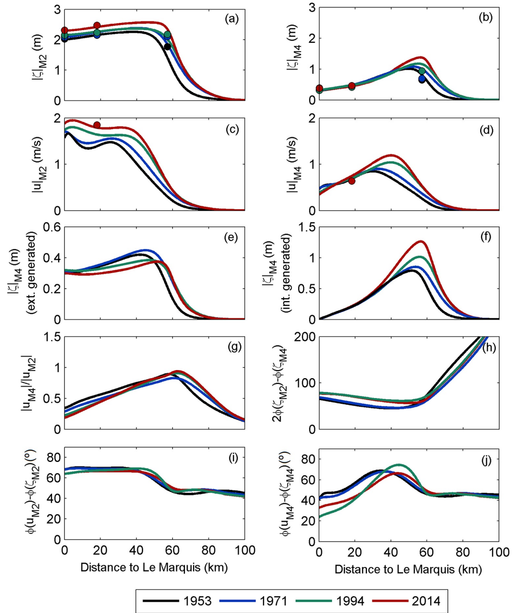
Figure 4. Multidecadal evolution of hydrodynamic parameters: water-level amplitude of the M_2 (a) and M_4 (b) components; current velocity amplitude of the M_2 (c) and M_4 (d) components; water-level amplitude of the (e) externally forced M_4 and the (f) internally generated M_4 ; horizontal tidal asymmetry distortion (g) and vertical tidal asymmetry direction (h); and phase differences between tidal currents and tidal height for M_2 (i) and M_4 (j) components. These results correspond to scenarios of spring tide (tidal range of 3.75 m at the estuary mouth) and low river discharge ( 125 \text{ m}^3/\text{s} ). Dots represent observations at (downstream to upstream) Le Marquis, Bordeaux, and Cadillac stations.
