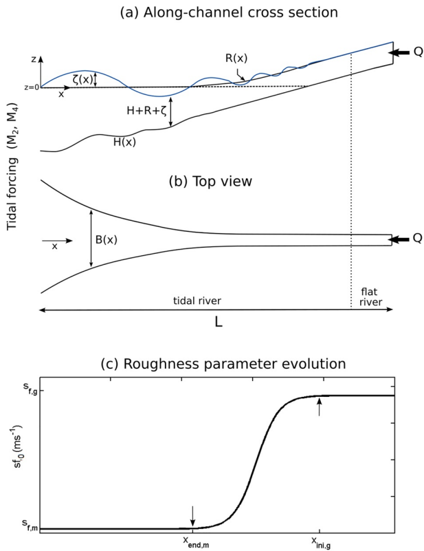
Figure 2. (a and b) Geometry of the tidal river in the idealized model. (c) Evolution of the partial slip parameter s_{f,0} over the longitudinal axis x , modeled by a hyperbolic-tangent function.
