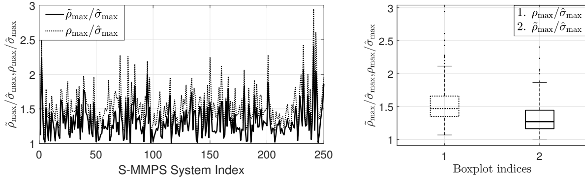
Fig. 1. Ratio of smallest upper bound to the growth rate of 250 well-defined, arbitrarily switching MMPS systems
