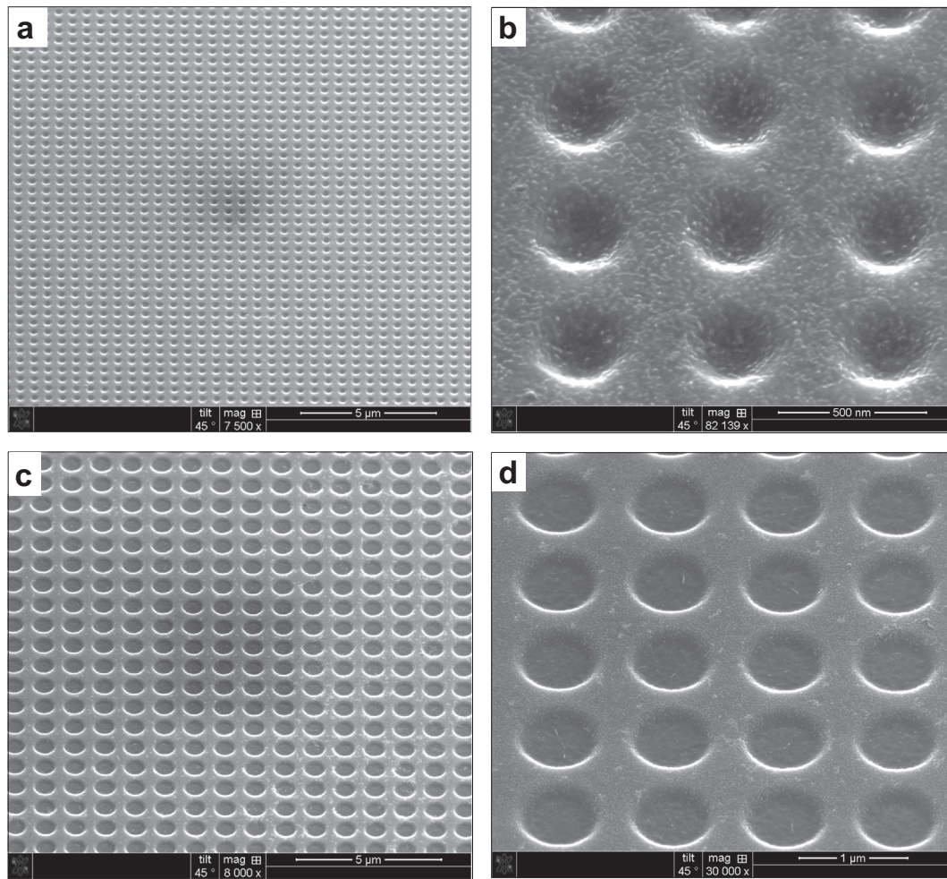
Fig. 6. Scanning electron micrographs of the titanium patterns (tilt 45°) produced using the Al/SiO 2 etch mask and three different etching steps: a and b arrays of small pits with ca 300 nm diameter at two different magnifications; c and d arrays of large pits with ca 714 nm pits at two different magnifications.
