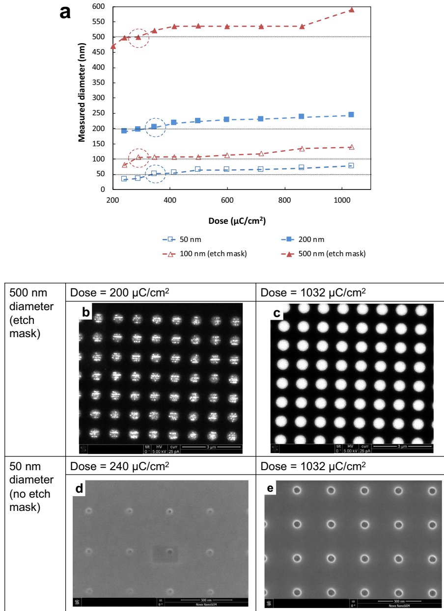
Fig. 4. (a) Effects of the applied dose on pattern diameters after development of the AR P-6200.04 resist (encircled values represent the optimum doses and the dotted horizontal lines represent the designed diameters); (b–e) examples of the patterns produced with low and high doses.
