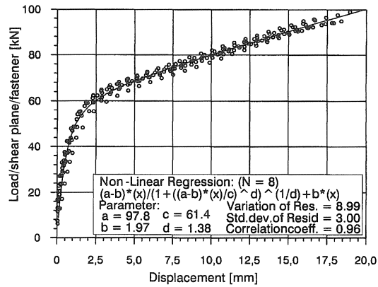
Fig. 26. Jaspart's model fitted to the test results: Knee joints with 35 mm tubes, Series 24 and 25.
