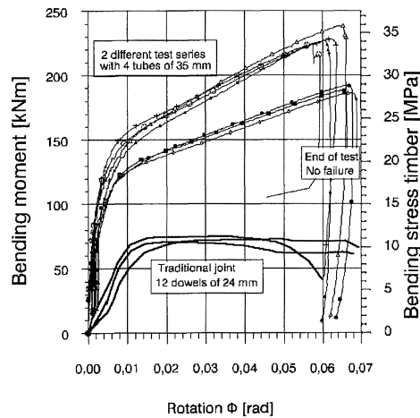
Fig. 24. Moment-rotation results of knee joints bottom test series: Non reinforced joints with traditional 24 mm diameter dowels top two test series: Dow reinforced joints with expanded 35 mm diameter tube fasteners, top: test Series 24 and below test Series 25.
