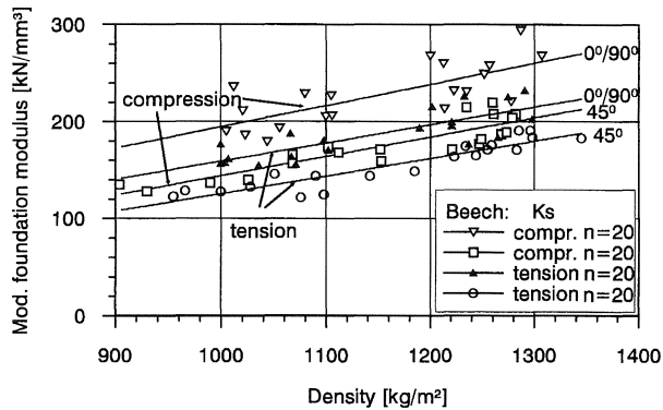
Fig. 10. The foundation modulus of dvw versus density and load to grain direction.
