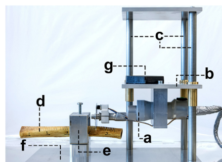
Fig. 1. Experimental setup used to cut the bone, the setup consisted of: an oscillating saw (a) fastened to a vertical sliding platform (b) guided by 3 stainless steel rods and brass sliding bearings (c). The bone specimen (d) was clamped in a v-groove holder (e), that was connected to an aluminium base plate (f). Interchangeable weights could be attached to the platform (g). The sawing action is further illustrated in Fig. 2.
