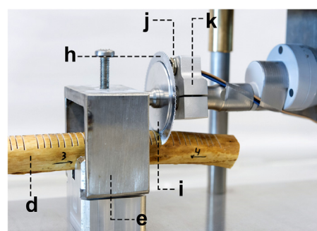
Fig. 2. Close-up of the saw blade and bone specimen, the setup consisted of: the bone specimen (d) was clamped in place by the v-groove holder (e). The saw blade (h) cut in the bone until the stopper (i) reached the bone for a consistent depth of cut. The Hall-effect sensor (j) acted as a tachometer, and was clamped to the saw with an aluminium block (k).
