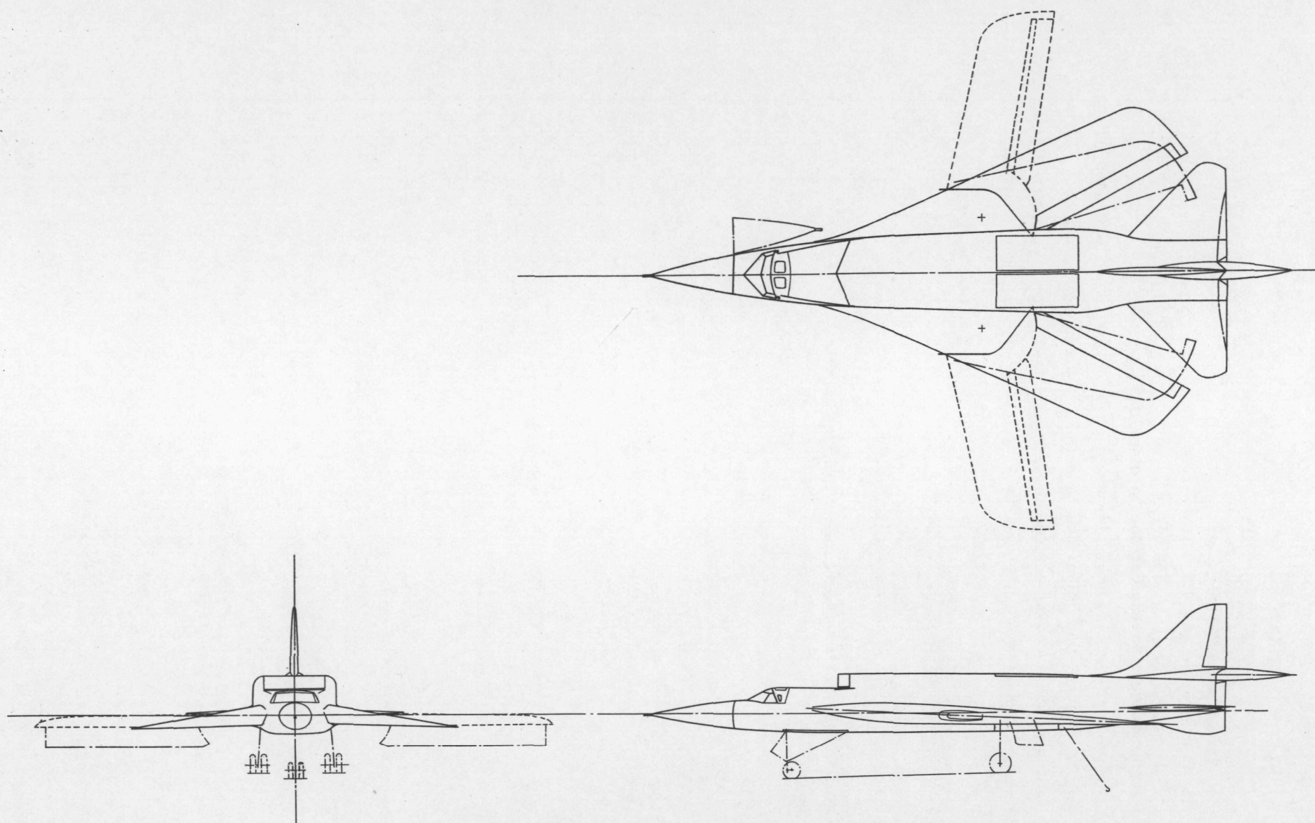
FIG.1. G.A. OF S 64 NAVAL STRIKE AIRCRAFT
