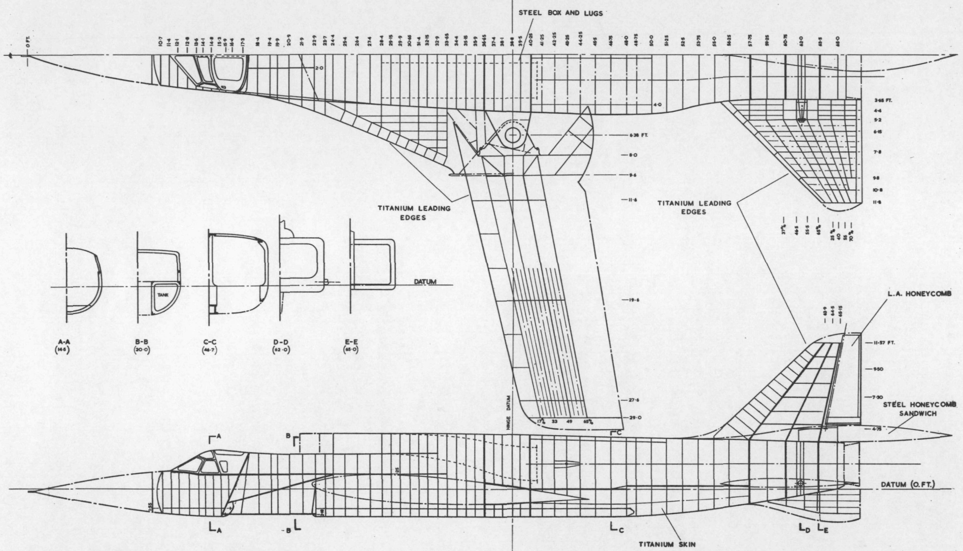
FIG. 18. STRUCTURAL LAYOUT
