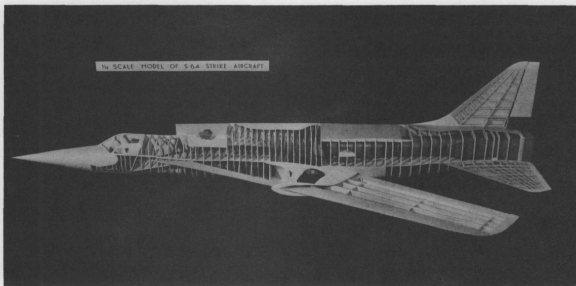
FIG. 3. PHOTOGRAPH OF A STRUCTURAL MODEL
