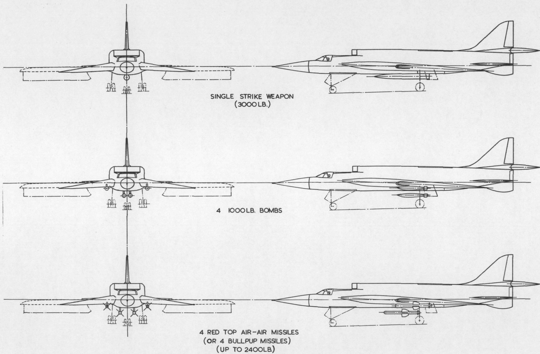
FIG. 5. TYPICAL WEAPON LOADS
