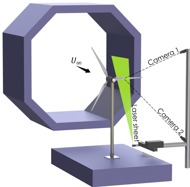
Figure 3. Experimental setup and measurement system.
