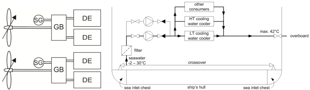
Figure 1.2 Block diagram of conventional diesel geared-drive propulsion system (left) and seawater cooling system (right) – copied from Klein Woud et al. [36] and [37] with permission.
