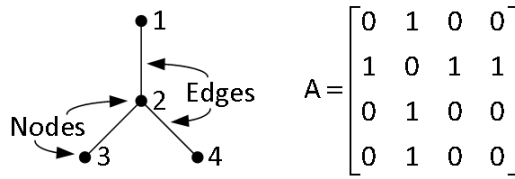
Figure 3.1 Example of a small undirected network ( nn = 4 ) incl. adjacency matrix A .
