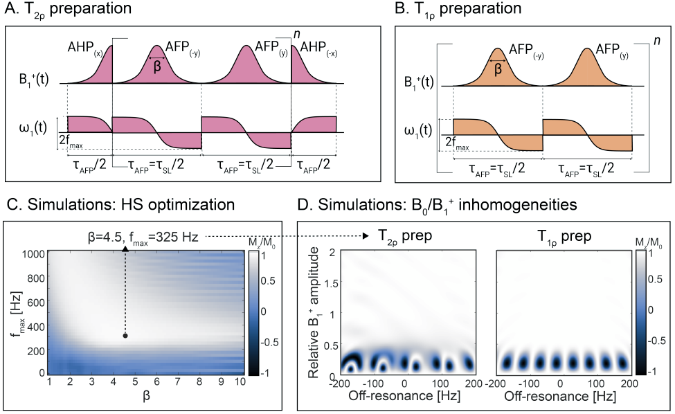
Figure 6.1 : A) T_{2\rho, \text{adiab}} preparations consist of an AHP pulse ( \tau_{\text{AHP}} = 10 ms) as flip-down, n pairs of HS AFP pulses ( \tau_{\text{AFP}} = 20 ms), and a time-reversed flip-up AHP pulse. Phase cycling is used to compensate for B_0/B_1^+ inhomogeneities. B) T_{1\rho, \text{adiab}} prep consists of n identical AFP trains. C) Bloch simulations of the preparation efficiency ( M_z/M_0 ) over a design region of off-resonances \in [-200, 200] Hz and relative B_1^+ \in [0.5, 1] . D) M_z/M_0 for the optimal parameters ( \beta = 4.5 and f_{\max} = 325 Hz) is shown for a range of off-resonances \in [-200, 200] Hz and relative B_1^+ \in [0.5, 1] . Faint diagonal patterns of suboptimal efficiency are visible for T_{2\rho, \text{adiab}} preparations.
