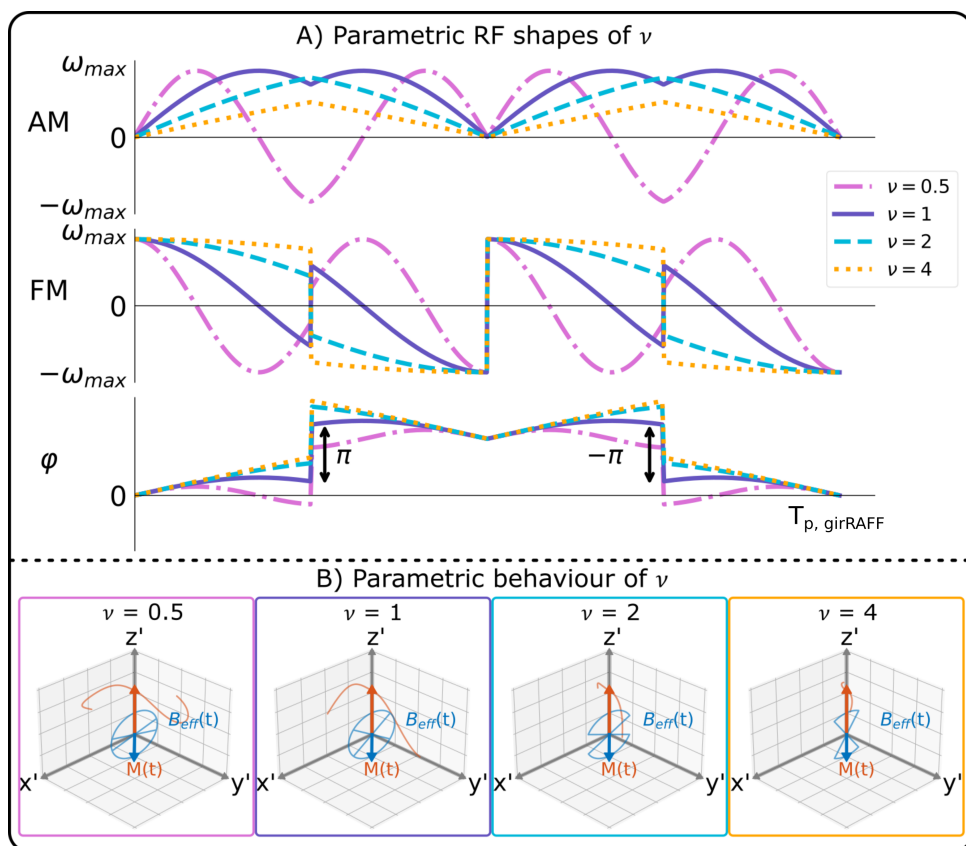
Figure 7.33 : A) Radiofrequency shapes: amplitude modulation, frequency modulation, and phase for the changing parametric behavior of \nu with respect to RAFF ( \theta = 0^\circ , \nu = 1 and \rho = 1 ) as default. B) Corresponding magnetization behavior for all RF shapes in the first rotating frame. Indicating the magnetization vector ( M(t) , orange) with its trajectory and the effective field ( B_{eff}(t) , blue).
