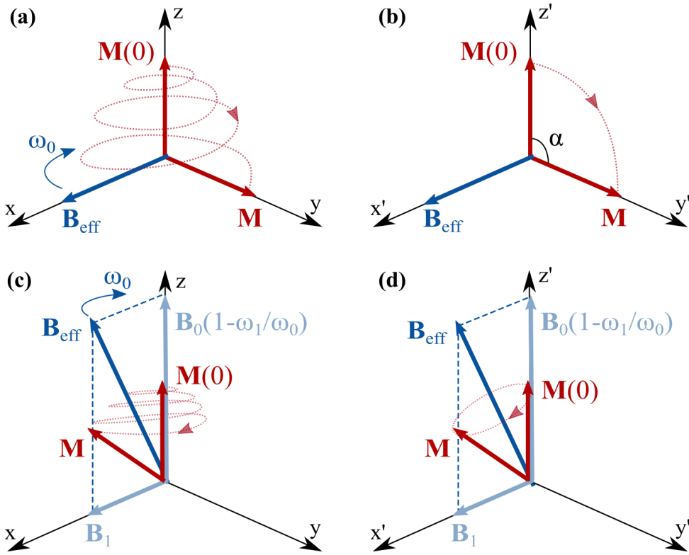
Figure 2.4 : On-resonance 90^\circ excitation pulse ( \mathbf{B}_{\text{eff}} = \mathbf{B}_1 , \omega_1 = \omega_0 ) tipping the magnetization to the transverse plane, as viewed in the (a) laboratory and (b) rotating frame of reference (RFR). (c, d) Off-resonance excitation pulse ( \omega_1 \neq \omega_0 ), causing \mathbf{B}_{\text{eff}} to be strongly angled towards the z-axis, preventing full excitation.
