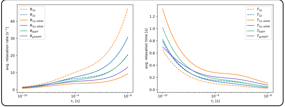
Figure 7.55 : Rotating frame relaxation rates and relaxation times, for conventional continuous wave T_{1\rho} and T_{2\rho} at 500 Hz, adiabatic T_{1\rho,adiab} and T_{2\rho,adiab} , and RAFF and girRAFF, for various correlation times. The relaxation rates were derived from second-order perturbation theory for the case of dipole-dipole interaction of like spins. RAFF and girRAFF show similar relation trends as T_{1\rho,adiab} and T_{2\rho,adiab} , where RAFF falls between T_{1\rho,adiab} and T_{2\rho,adiab} and girRAFF falls between T_{1\rho,adiab} times and RAFF. Continuous wave T_{1\rho} and T_{2\rho} trends show less similarity with RAFF and girRAFF.
