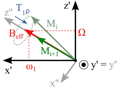
Figure 8.1 : The effective field B_{\text{eff}} and the magnetization vector M in the first rotating frame. In the second rotating frame, B_{\text{eff}} is aligned with the z -axis. In this figure, the magnetization vector evolves from M_i to M_{i+1} , following the effective field. It also shortens due to T_{1\rho} relaxation.
