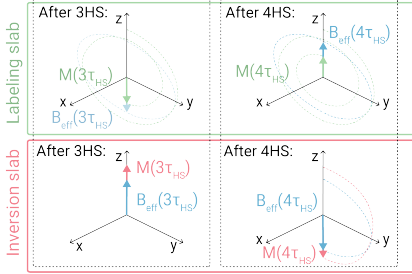
Figure 5.1 : A) T_{1\rho, \text{adiab}} preparation module, consisting of a train of hyperbolic secant (HS) pulses, with corresponding amplitude and frequency modulation functions. A slice-selective gradient ( G_{ss} ) is used on all but the last HS to achieve dark-blood (DB) contrast. B) Magnetization ( M ) trajectories for spins in the labeling and inversion slabs during the slice-selective HS pulses (left) and at the end of the entire preparation module (right). Spins in the inversion slab only experience the last non-selective HS pulse and are effectively inverted at the end of the preparations, while spins in the labeling slab experience an even number of HS pulses, yielding a final T_{1\rho, \text{adiab}} -prepared positive longitudinal magnetization. C) Slice profile obtained with the DB- T_{1\rho, \text{adiab}} -preparations, with G_{ss} chosen orthogonal to the imaging slice orientation to visualize the labeling slab.
