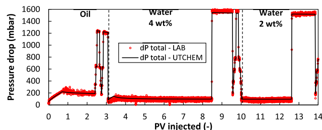
Figure 4. Simulated and measured total pressure drop ( dP total) profiles for primary drainage (oil) and waterflooding (water) for simulation 3. Approximately 3.0 pore volume (PV) of oil was injected prior to waterflooding.
