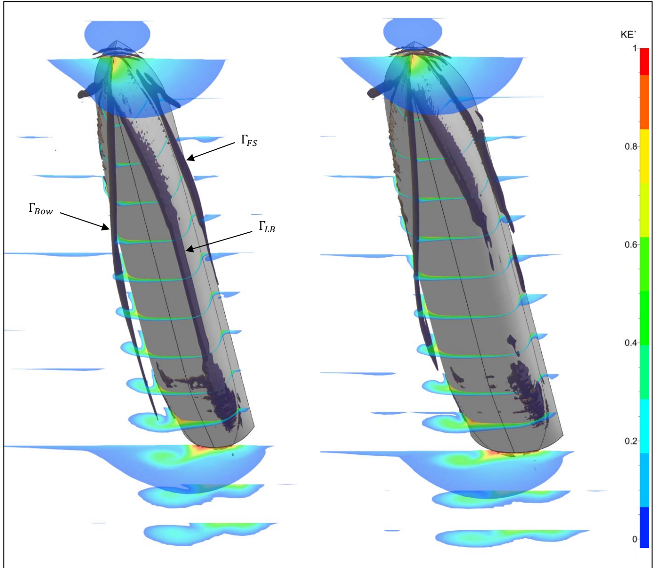
Figure 7: Numerical simulation for two wind-assist hulls with 12 knots boat speed and leeway angle equal to 9°. The orientation of the coordinate system is such that the direction of vessel motion is toward the top of the page. Longitudinal vortices are identified in dark purple, while the (normalized) fluid kinetic energy is given on transverse sections. The left hull has 20% larger T/L compared to the right hull (for the same displacement).
