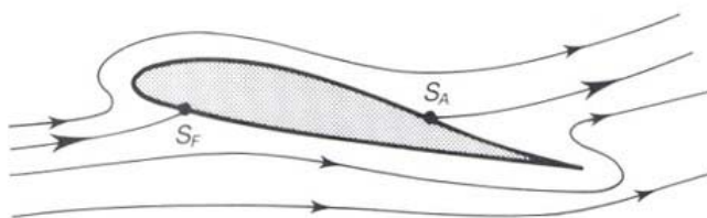
Figure 3: Wing section at t=0^+ , immediately following an impulsive acceleration. The after stagnation point is located on the suction side. Flow passes around the trailing edge with infinite velocity.
