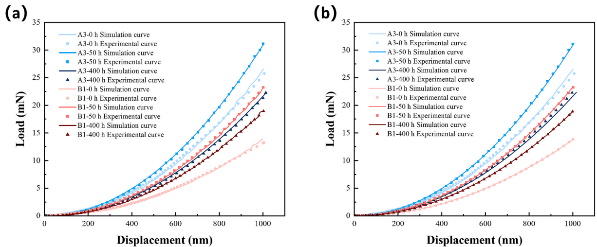
Fig. 22. Comparison of load-displacement curves predicted by the elastoplastic model of Cu-Ag composite sintered joints with experimental results: (a) n = 0 , (b) n \neq 0 .
