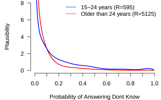
(a) Age subgroups for “don’t know” in the survey Politics (Cliff's \hat{\delta}_P = 0.28 , 99% C.I. = [0.22, 0.34])
