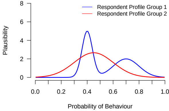
(a) Respondent profiles for group 1 (mean=0.55) and group 2 (mean=0.45) with reference Cliff's \delta = 0.29
