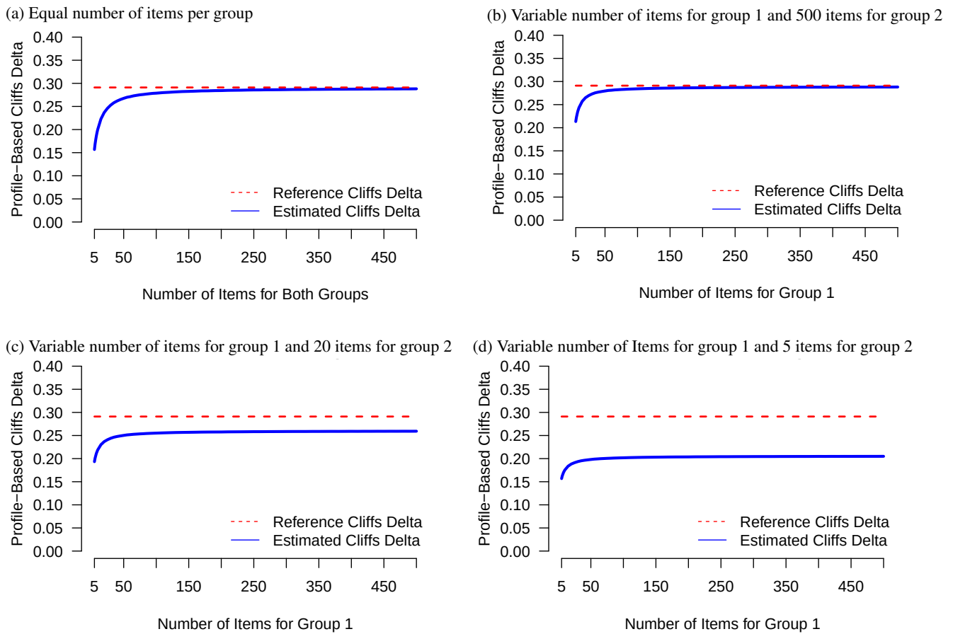
Figure 5. Estimated profile-based Cliff's \hat{\delta} for two distributions from 500 respondents with varying numbers of items per group and \delta = 0.29 .
