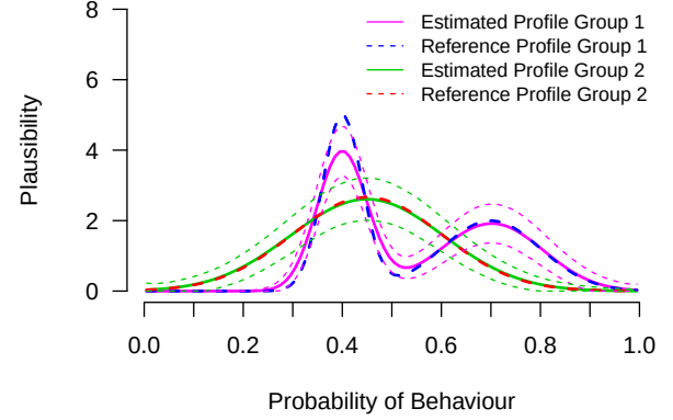
Figure 4. Estimated respondent profiles and their statistical properties for group 1 (mean=0.55) and group 2 (mean=0.45) with estimated profile-based Cliff's \hat{\delta} = 0.29
