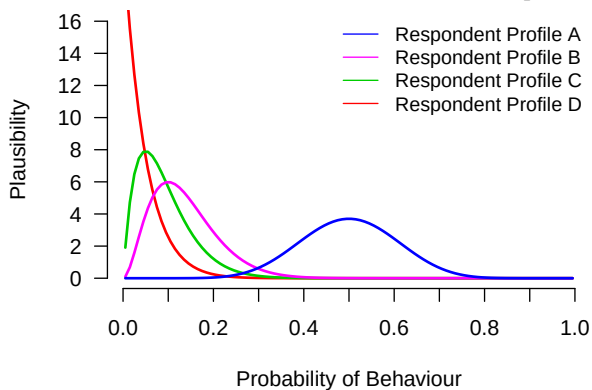
(a) The same number of items and different behaviour probability
