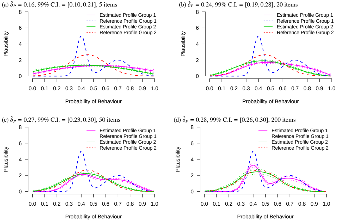
Figure 6. Estimated respondent profiles and their statistical properties for varying numbers of items for both groups of respondents (reference Cliff's \delta = 0.29 ).
