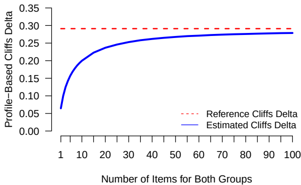
(a) 1 through 100 items per respondent (500 respondents in both groups)
