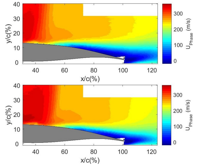
Figure 13: Phase average of the U component of the velocity for the straight (2% c ) UGF configuration, with the shock in the most upstream position (1) (top figure) and downstream position (5) (bottom figure)
