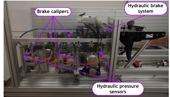
Fig. 6. Electro-hydraulic brake system test bench.
