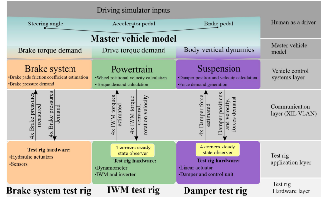
Fig. 3. Model architecture.
