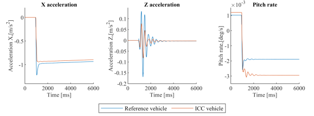
Fig. 8. Results of the simulation of reference vehicle and vehicle with integrated chassis controller for straight-line braking maneuver.
