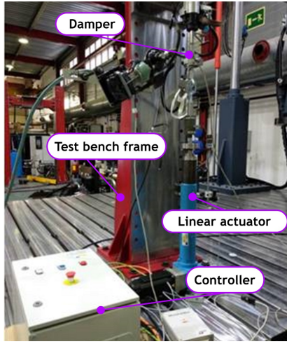
Fig. 7. Suspension test bench.
