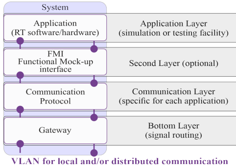
Fig. 4. Model architecture.
