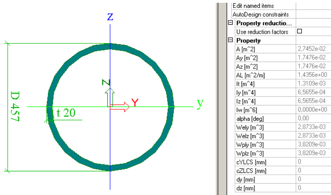
Figure B - 36 Rest braces - Design with CHS members and S355 steel grade only, case (b), U.C. = 0.81
