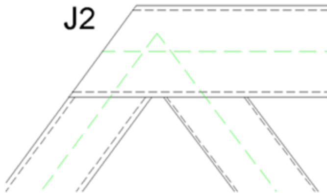
Figure B - 9 Critical joint 2 configuration, K- gap joint
