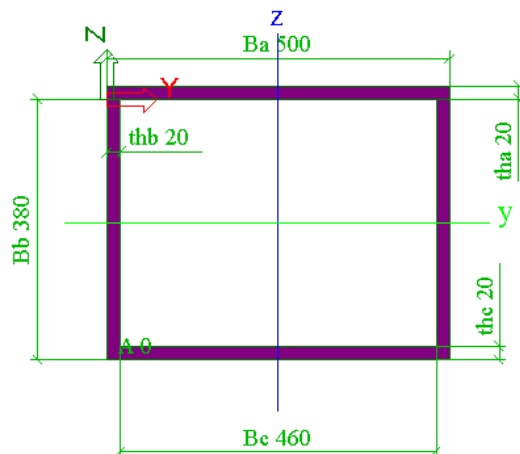
Figure B - 19 End (compression) braces, U.C. =0.91
