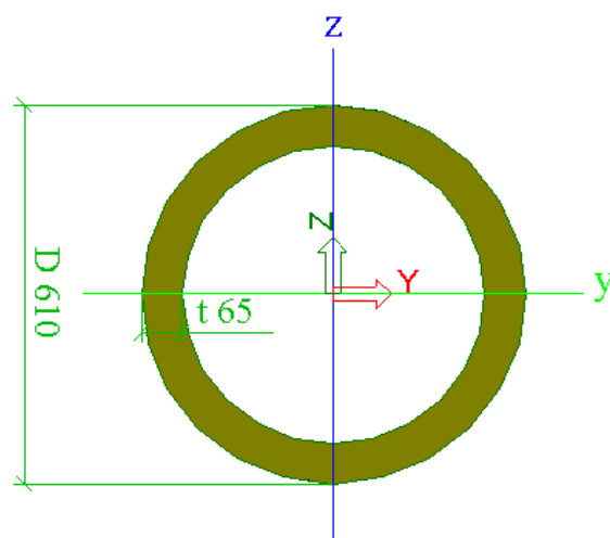
Figure B - 30 Bottom chord- Design with CHS members and S355 steel grade only, case (a), U.C. =0.91
