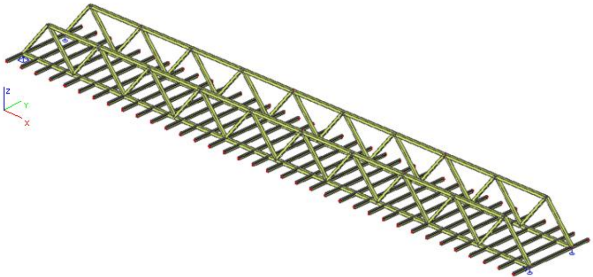
Figure 5.8 3D FEM model in “Scia Engineer”, L/D = 15 , L_i = 10.5 m
