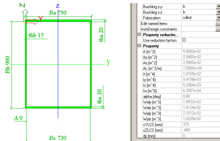
Figure A - 16 Bottom chord cross section, Truss 1-Scia Engineer
