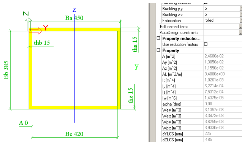
Figure A - 14 Brace cross section, Truss 1- Scia Engineer
