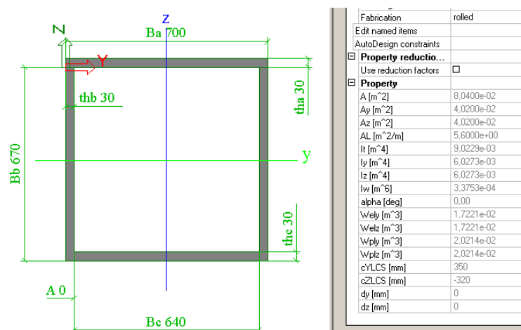
Figure A - 46 Figure 11 Arch, Arch 2- Scia Engineer
