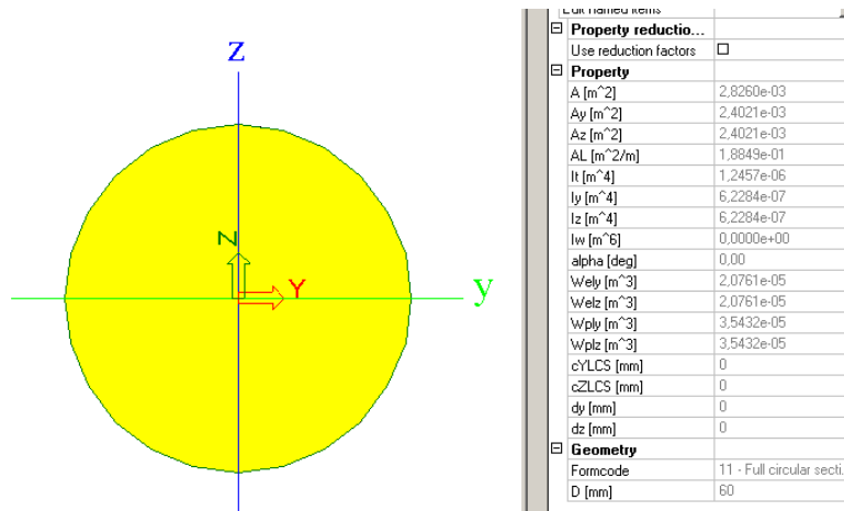
Figure A - 38 Vertical hangers, Arch 1- Scia Engineer
