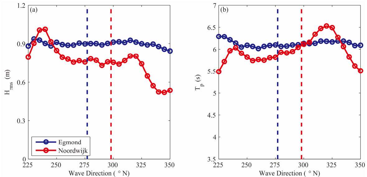
Figure 4. Comparison of the time-mean H_{rms} wave height (a) and the time-mean peak wave period (b) at Noordwijk and Egmond as a function of the incident wave direction. The vertical lines indicate the shore normal orientation for both sites.
