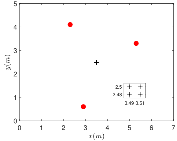
Fig. 1: Acoustic scene. The three red circles denote the sources. The cross in the center denotes the set of microphones. A zoom-in of that set of four microphones is provided in the little square.
