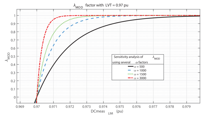
FIGURE 4. Exponential response presenting the non-linear relationship between \lambda_{MOD} and DC_{measLIM} for different \alpha values.
