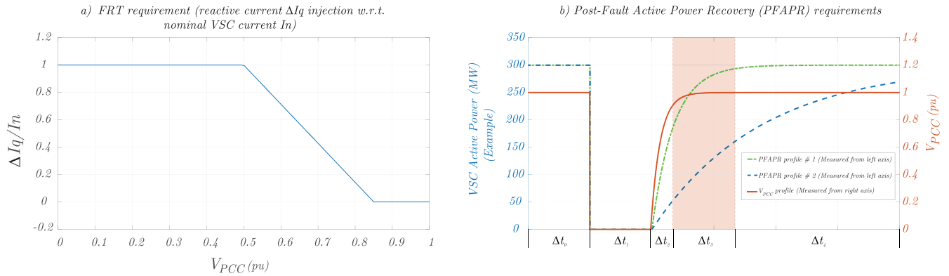
FIGURE 2. VSC unit requirements for the FRT and the PFAPR function. Fig. 2a shows the level of reactive current injection ( \Delta I_q w.r.t. to the nominal I_n VSC AC current) depending on the voltage ( V_{PCC} ) dip experienced in the AC network. Fig. 2b shows active powers and V_{PCC} voltage profiles during a pre-fault ( \Delta t_0 ), fault ( \Delta t_1 ), and post-fault ( \Delta t_2 , \Delta t_3 , \Delta t_4 ) time periods.
