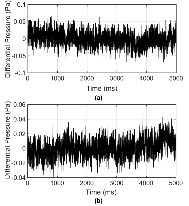
Fig. 16. Measured RMS pressure noise of the sensing system with a shorted (0 Pa) input for (a) LTC6363 and (b) THS4551.
