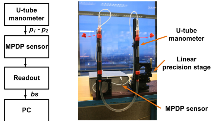
Fig. 13. Differential pressure measurement setup.
