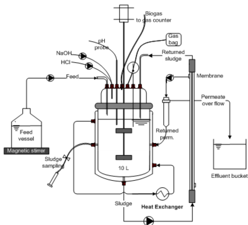
Figure 4.1 – AnMBRs experimental set-up
