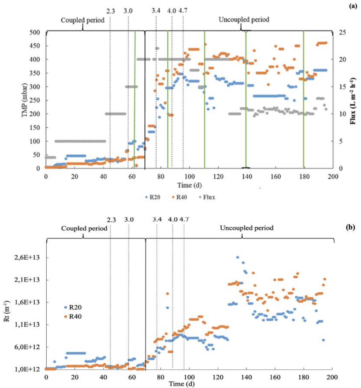
Figure 4.6 – (a) Flux L / (m^2 \cdot h) and TMP (mbar), and (b) R_{total} values over time for the R20 and R40 reactors. The dotted lines indicate the applied OLR ( g \text{ COD} / (Ld) ), and the green lines indicate the CIP interventions carried out in the reactors.
