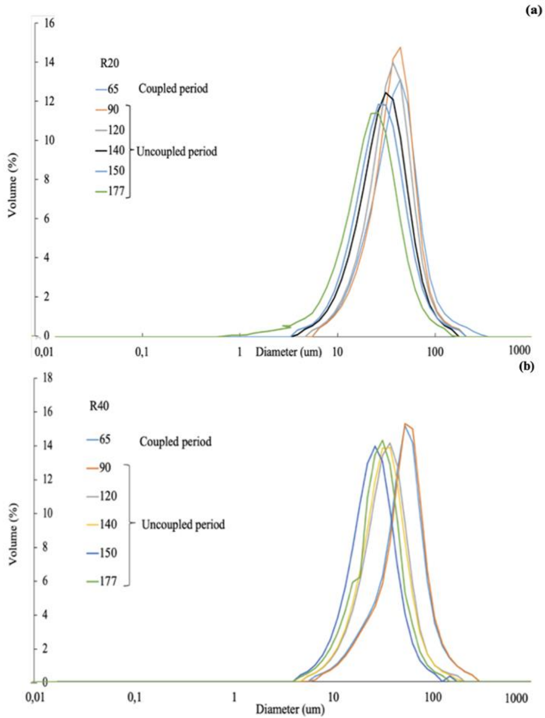
Figure 4.3 – PSD over operational time for (a) R20, and (b) R40 reactors over time.
