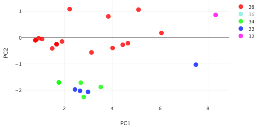
Figure 19. Scatter Plot of Data with PC 1 and PC 2 as the axis (4 clusters are presented – 36 is not presented)
