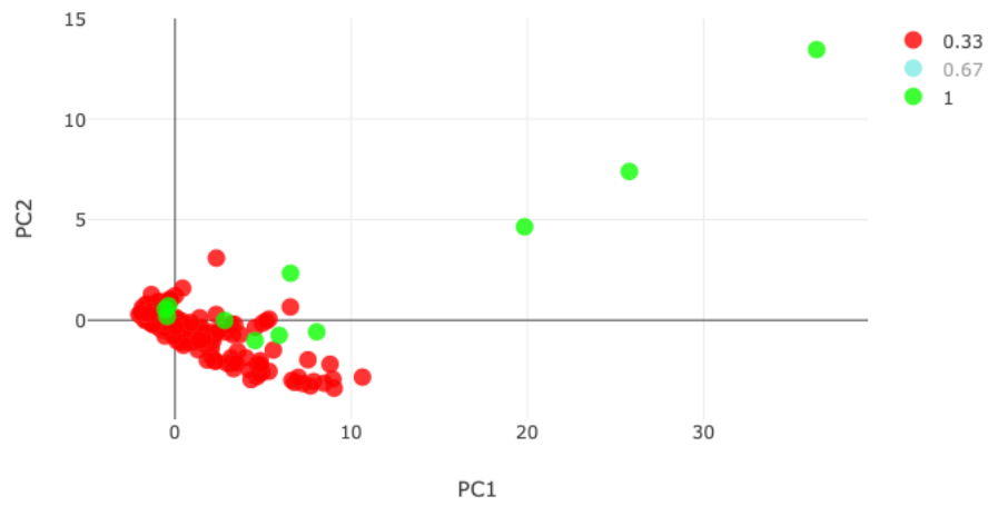
Figure 15. Scatter Plot of Data with PC 1 and PC 2 as the axis (three multiplexity are presented – 0.33 and 1)
