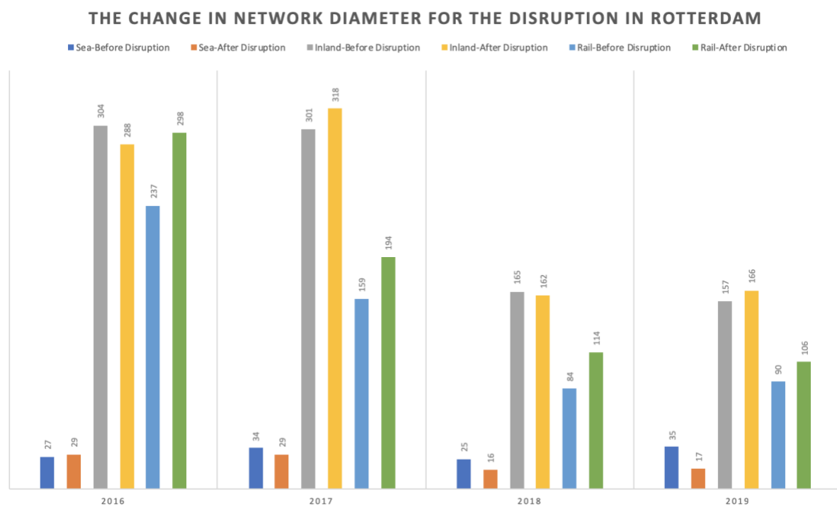
Figure 61. The Change in The Network Diameter for The Disruption in Rotterdam
