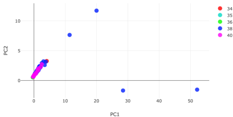
Figure 26. Scatter Plot of Data with PC 1 and PC 2 as the axis (Full Clusters are presented)
