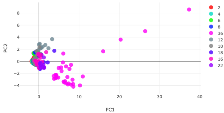
Figure 20. Scatter Plot of Data with PC 1 and PC 2 as the axis (all clusters)
