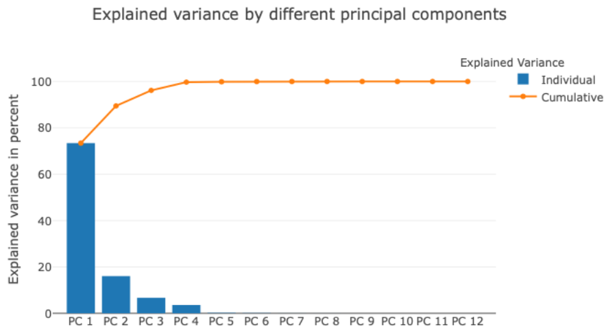
Figure 25. The rank of Metrics based on Explained Variance – Clustering by 5 Highest K-Core Value
