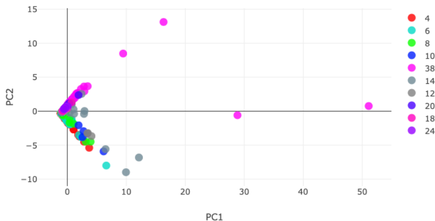
Figure 28. Scatter Plot of Data with PC 1 and PC 2 as the axis (4 clusters are presented – 36 is not presented)
