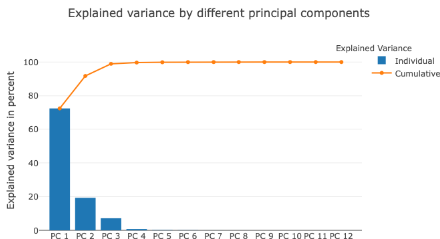
Figure 22. The rank of Metrics based on Explained Variance – Clustering by Multiplexity
