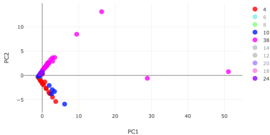
Figure 29. Scatter Plot of Data with PageRank and Eigenvector as the axis (5 clusters are presented – 2,4,6,22,36)
