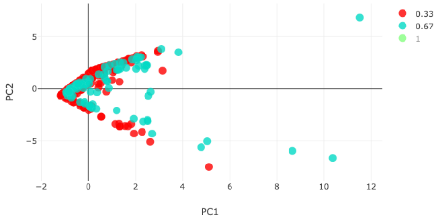
Figure 24. Scatter Plot of Data with PC 1 and PC 2 as the axis (two multiplexity are presented – 0.33 and 0.67)
