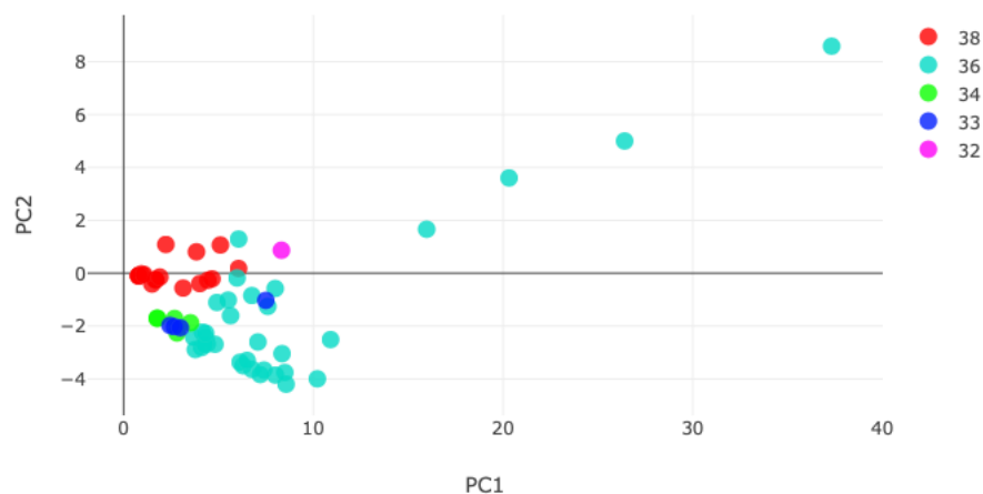
Figure 18. Scatter Plot of Data with PC 1 and PC 2 as the axis (Full Clusters are presented)
