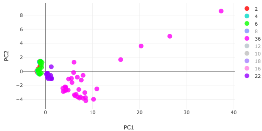
Figure 21. Scatter Plot of Data with PC 1 and PC 2 as the axis (5 clusters are presented – 2,4,6,22,36)
