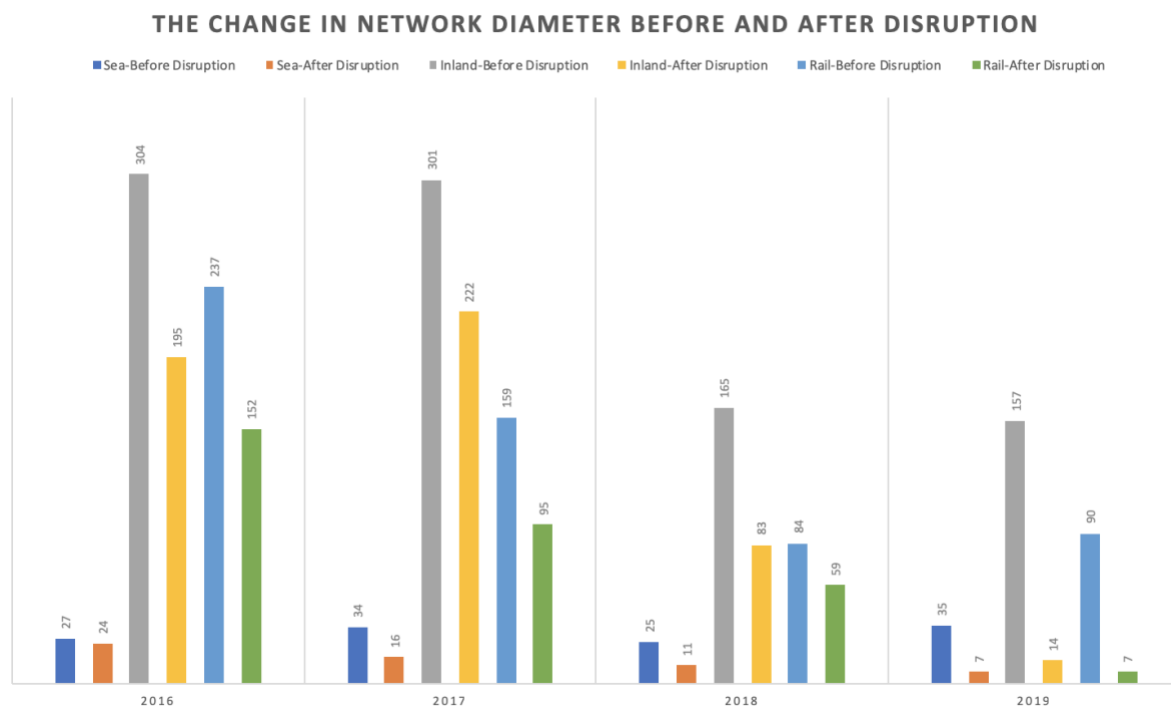
Figure 58. The Change in The Network Diameter Before and After Disruption
