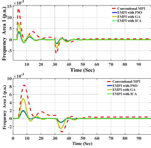
Fig. 10. Comparisons between MPI controller scenarios on classical two-area LFC model for outputs: (a) \omega_1 , (b) \omega_2 .
