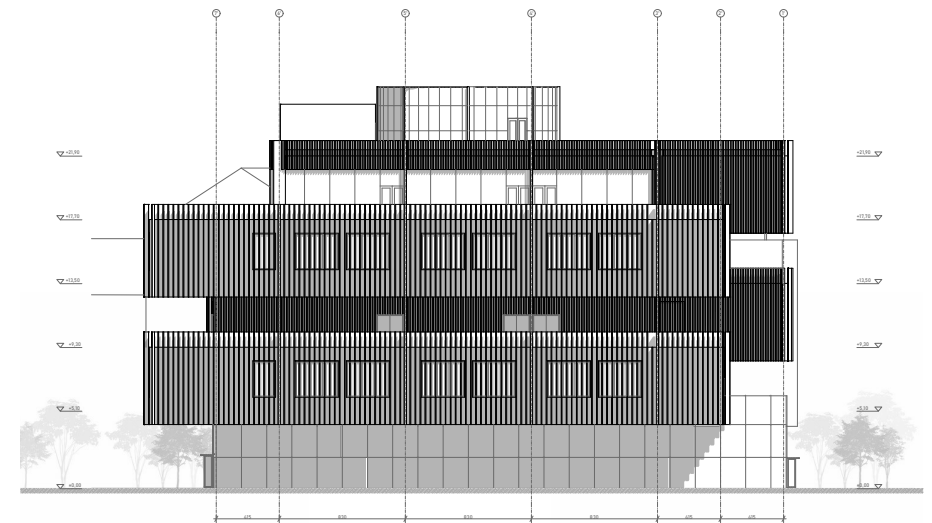
South-West Facade
