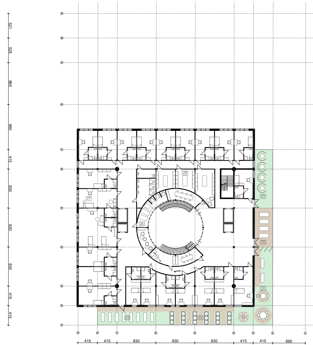
Floor +3 1:200
