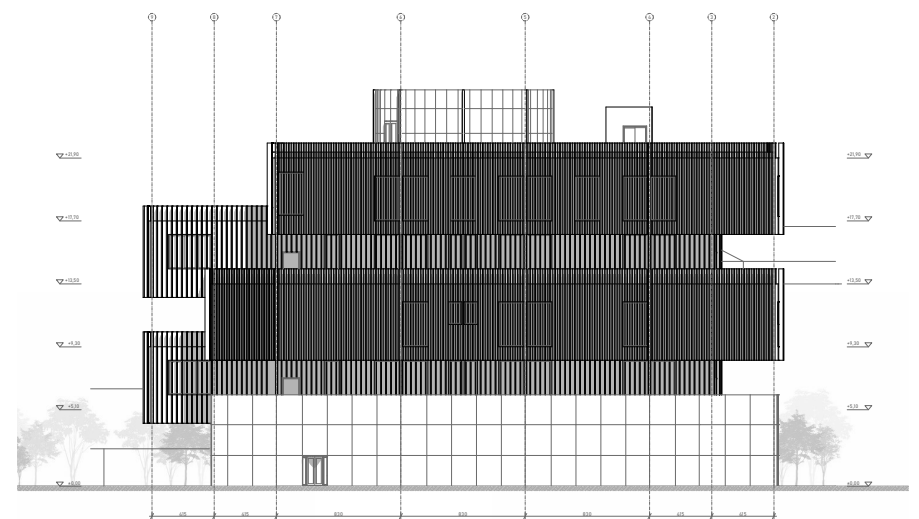
South-East Facade
