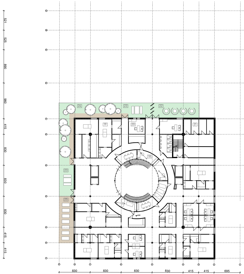
Floor +2 1:200
