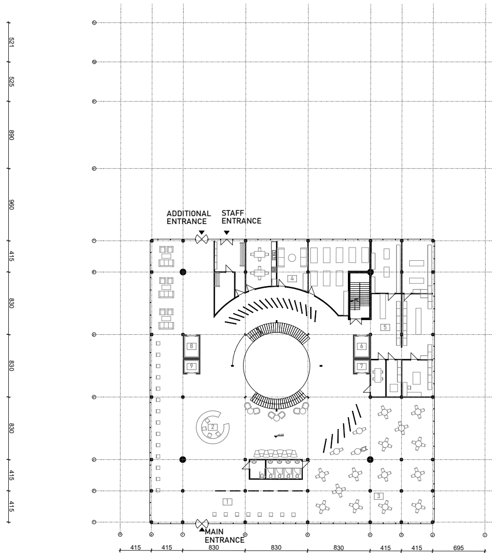
Ground Floor 1:200
