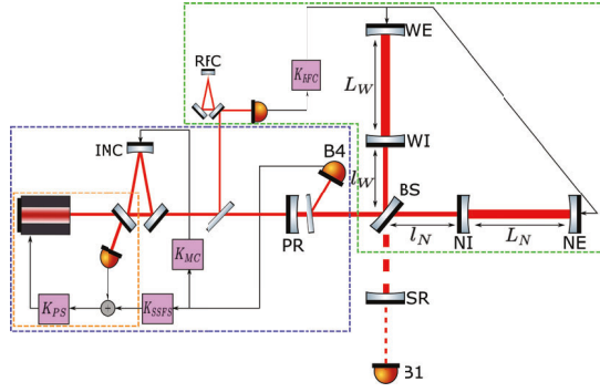
Fig. 1. The optical configuration of AdV, including the control scheme for the Common Arm. The B1 photodiode measures the interference pattern between the two arms ( L_W + L_W and L_N + L_N ), which change in length with opposite signs when a GW passes. The two arms L_W and L_N are 3 km long.
