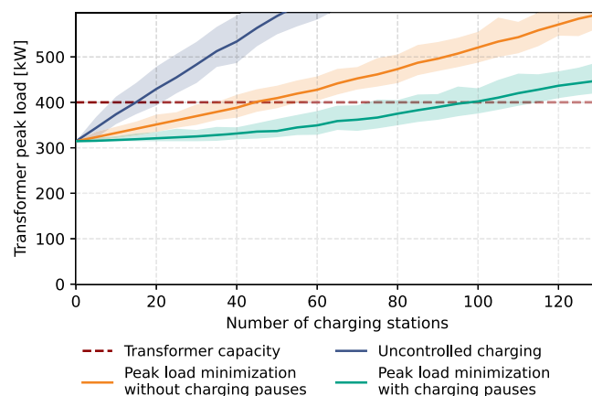
Fig. 5 | Peak transformer load values in a one-year assessment timeframe when applying a peak transformer load minimization algorithm to a different number of installed on-street charging stations in one residential LV grid in the city of Utrecht, the Netherlands. The analysis is repeated 100 times for each considered number of EV charging stations, with a randomly sampled subset of EV charging stations in each run. The line shows the average outcome for all model runs and the shaded area shows the 95% confidence interval. Source data are provided as a Source Data file.
