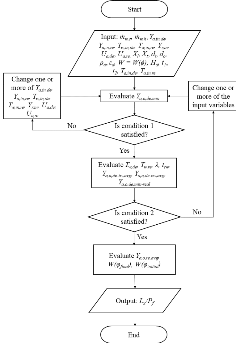
Figure 4: Flow-chart summarizing the feasibility check and design methodology
