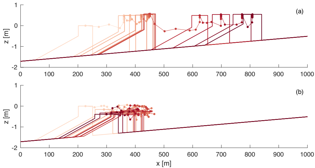
Fig. 10. Chenier evolution over 10 years, under stochastic boundary conditions. One profile per year is pictured, in increasingly darker shades of red. The position of the chenier center is indicated with a dot for each month. Panel (a) shows a scenario without phase lag ( \theta = 0 min) or storm reset ( \Delta x_{st} = 0 m). Panel (b) shows a scenario with a phase lag of \theta = 5 min and a storm reset of \Delta x_{st} = 100 m. (For interpretation of the references to colour in this figure legend, the reader is referred to the web version of this article.)
