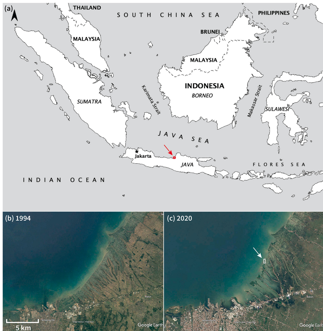
Fig. 1. (a) Map of the Java Sea and surroundings. The red dot on the north coast of Central Java indicates the location of the two inset photos in (b) and (c), which are satellite images of the coastline of Demak in 1994 and 2020 respectively (Google Earth, 2021). They highlight the extreme coastal erosion and coastline retreat in this area, as well as the rapid development of Semarang in the south. The white rectangle in (c) indicates the location of the zoomed satellite images in Fig. 2a-d. (For interpretation of the references to colour in this figure legend, the reader is referred to the web version of this article.)
