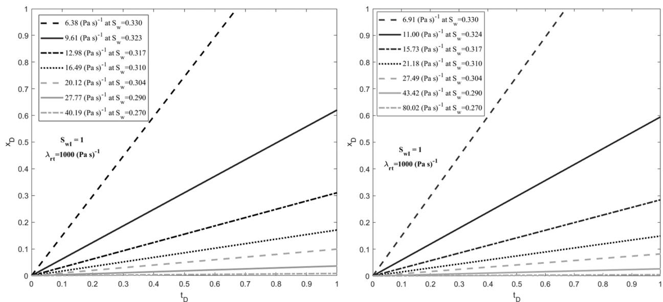
Fig. B.1. x_D vs t_D diagrams corresponding to gas injection excluding the NZ correction (on the left) and including the NZ correction (on the right). Values of total relative mobility in (\text{Pa s})^{-1} are given for the initial condition and selected characteristics.
