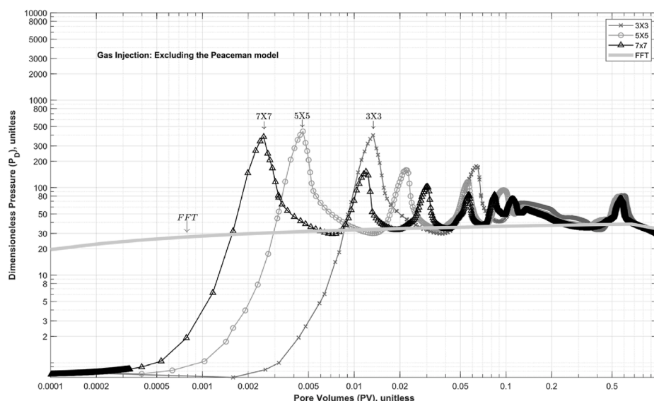
Fig. 14. Fractional-flow-theory calculations and simulations of gas injectivity obtained excluding both the Peaceman model and the NZ correction.
