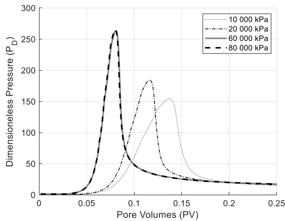
Fig. 6. Effect of reservoir pressure on the estimated injectivity during gas injection in a fully surfactant-saturated reservoir: STARS simulation with the base-case grid.
