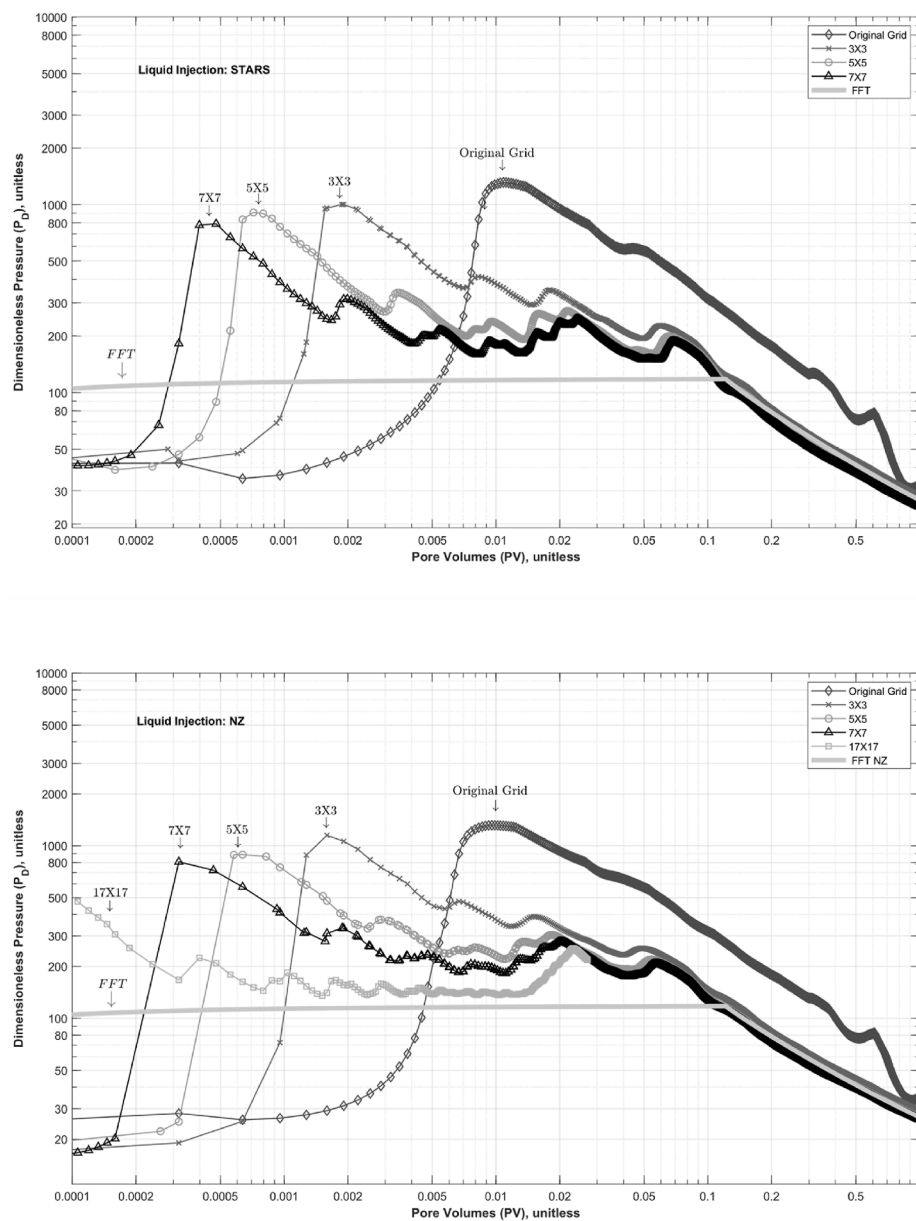
Fig. 13. Fractional-flow theory (FFT) calculations and STARS simulations of liquid injectivity at early times using the Peaceman model as implemented in the simulations. On the top plot we exclude the NZ correction, while on the bottom plot we include the NZ correction.
