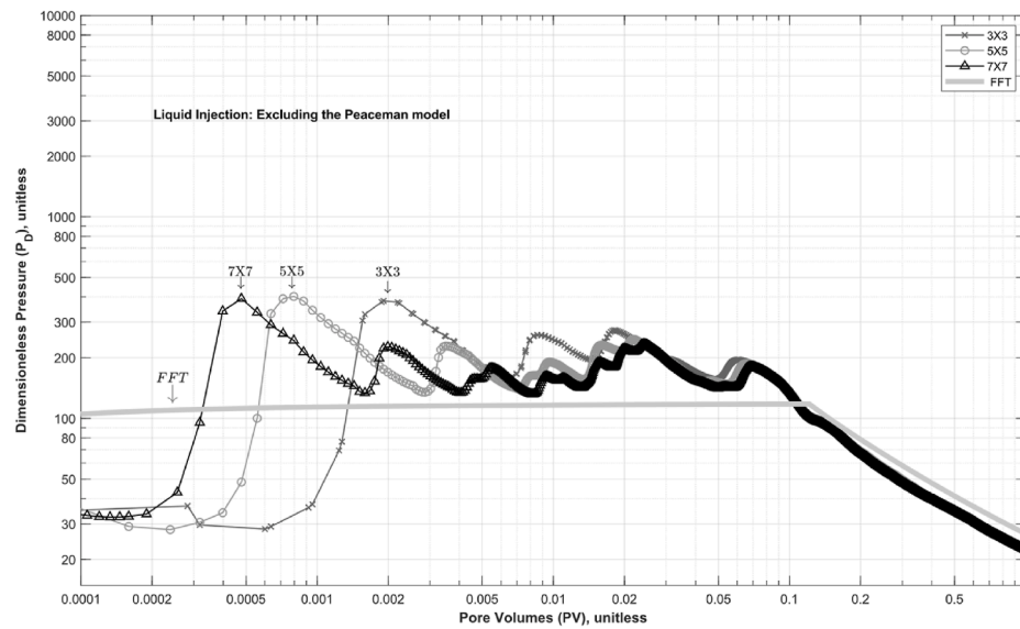
Fig. 15. Fractional-flow theory calculation and STARS simulations of liquid injectivity calculated excluding the Peaceman model. These cases also exclude the NZ correction.
