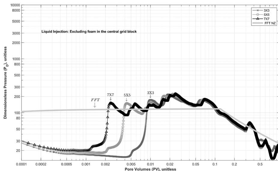
Fig. 18. Fractional-flow theory calculations and simulations of liquid injectivity at early times with foam excluded in the central grid block ( f_{mob} = 0 there).
