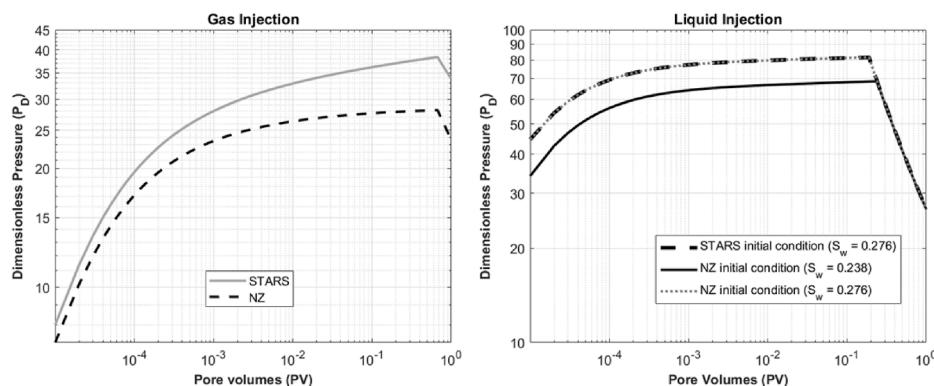
Fig. 8. Fractional-flow-theory calculations of gas and liquid injectivities. On the left, dimensionless pressure ( P_D ) during the injection of the first gas slug. On the right, P_D during the injection of the subsequent liquid slug.
