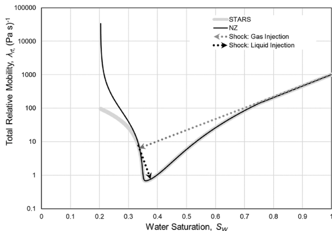
Fig. 7. Total relative mobility ( \lambda_{tr} ) of foam for the STARS model and considering the NZ correction.
