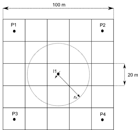
Fig. 2. Reservoir model used in simulations. P1 , P2 , P3 , and P4 denote four producing wells, and I1 represents the injection well. In our simulations, to reduce the fluctuations caused by subdividing the central grid block, we record the difference in pressure between the injection well and the center of the next grid block along the diagonal. For fractional-flow calculations, the outer radius is taken as r_o = \sqrt{2} \times 20 \text{ m} \approx 28.8 \text{ m} .
