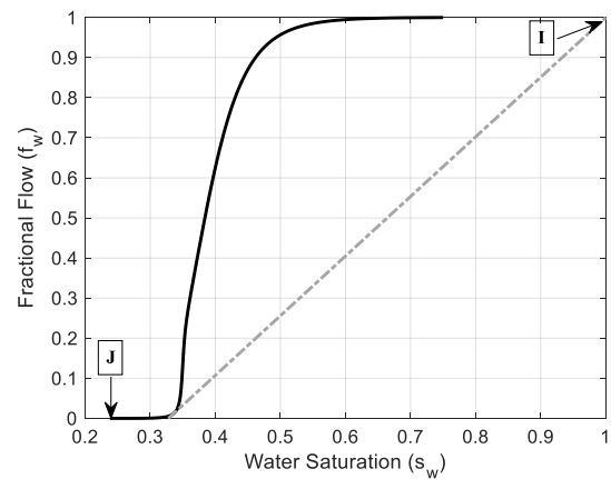
Fig. 4. Fractional-flow solution for injection of the first gas slug. Initial condition I and injection J correspond to 100% liquid saturation and 100% gas fractional flow, respectively. The dashed line represents the shock.
