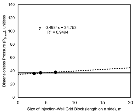
Fig. 19. Value of P_{D,ave} as a function of size of the injection-well grid block for the case that excludes foam at the well grid block. Black dots: simulation results. Dashed line: fit to simulation results. Black line, FFT result.
