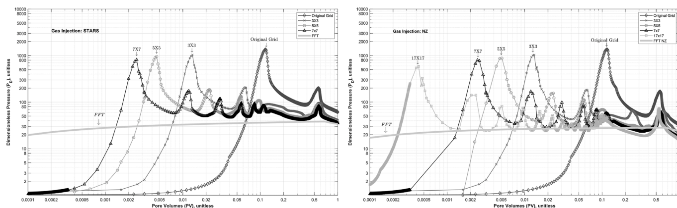
Fig. 9. Gas injectivity at early times for the original reservoir model and the three refined-grid cases ( 3 \times 3 , 5 \times 5 , and 7 \times 7 ) for the one that includes the STARS model but excludes the NZ correction (top plot) and four refined cases ( 3 \times 3 , 5 \times 5 , 7 \times 7 and 17 \times 17 ) for the scenario that includes the NZ correction (bottom plot). In these results, we use the injection-well pressure calculated using the Peaceman model implemented in STARS. To compare, we also plot the results of our FFT calculations excluding or including the NZ correction.
