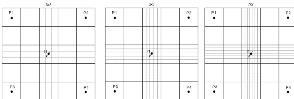
Fig. 3. Refined reservoir models used in simulations.
