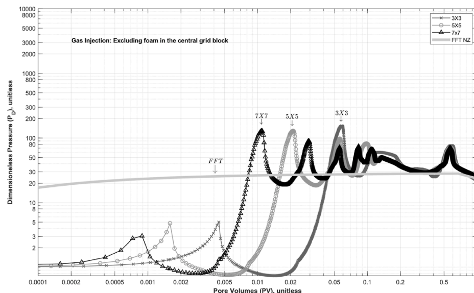
Fig. 17. Fractional-flow-theory calculation and simulations of gas injectivity at early times excluding foam in the central grid block ( fmmob = 0 ).
