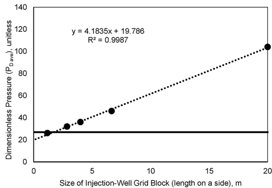
Fig. 12. Value of P_{D\text{ave}} as a function of size of the injection-well grid block for the case of Peaceman model, including NZ correction. Black dots: simulation results. Dashed line fit to simulation results. Black line, FFT result.
