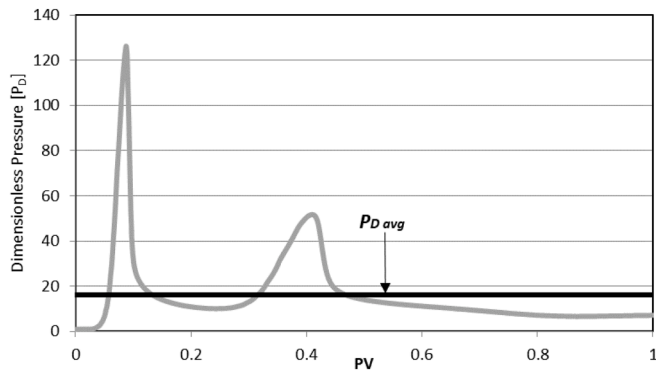
Fig. C.1. Illustration of the physical meaning of the average dimensionless pressure P_{D,avg} during gas injection in a simulation using the grid without refinement and excluding the Peaceman equation.
