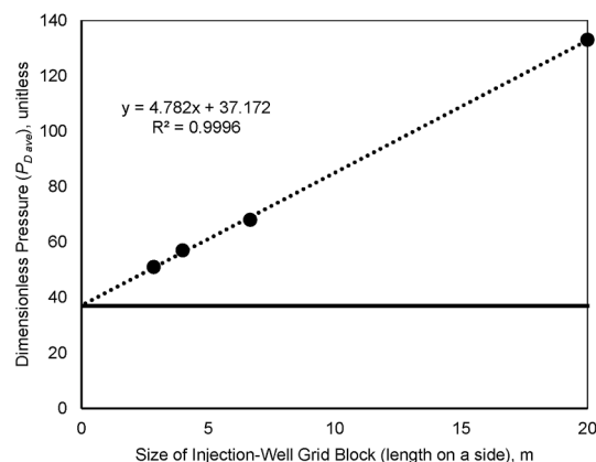
Fig. 10. Value of P_{D\text{ ave}} as a function of size of the injection-well grid block for the case of Peaceman model, no NZ or other modification. Black dots: simulation results. Dashed line fit to simulation results. Black line, FFT result.
