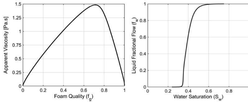
Fig. 1. On the left, plot of apparent viscosity versus gas fractional flow ( f_g ) (or “foam quality”) computed using the parameters listed in Table 1. On the right, liquid fractional flow ( f_w = 1 - f_g ) is plotted as a function of water saturation ( S_w ) using the same input parameters.
