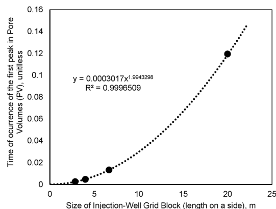
Fig. 11. Time of occurrence of the first dimensionless pressure peak as a function of size of the injection-well grid block for the case of Peaceman model, no NZ or other modification. Black dots: simulation results. Dashed line fit to simulation results.
