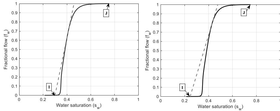
Fig. 5. Fractional-flow solutions for injection of a liquid slug after gas injection, assuming two initial water saturations S_{wi} of 0.3341 and 0.2421 in the near-well region. The slopes of the dashed lines represent the dimensionless velocities of the shocks.
