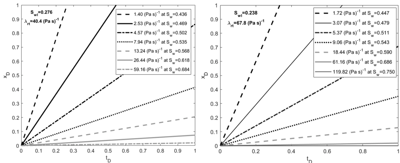
Fig. B.2. x_D vs t_D diagrams for liquid injection assuming an initial uniform water saturation on the left S_{wi} = 0.276 and on the right S_{wi} = 0.238 . Values of total relative mobility in (\text{Pa s})^{-1} are given for the initial condition and selected characteristics.
