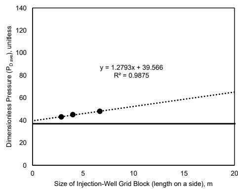
Fig. 16. Value of P_{D,avg} as a function of size of the injection-well grid block for the case that excludes both the Peaceman model and NZ correction. Black dots: simulation results. Dashed line fit to simulation results. Grey line, FFT result.
