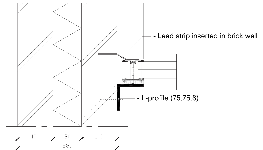
detail J (1:5)
