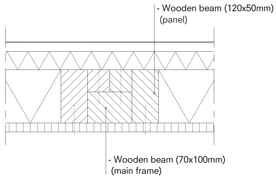
detail I (1:5)
