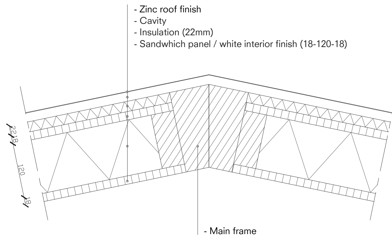
detail L (1:5)
