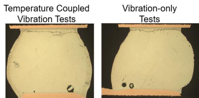
Fig. 22: Failure Analysis Results Comparing BL [VIBR+TC] vs. BL [VIBR] tests
