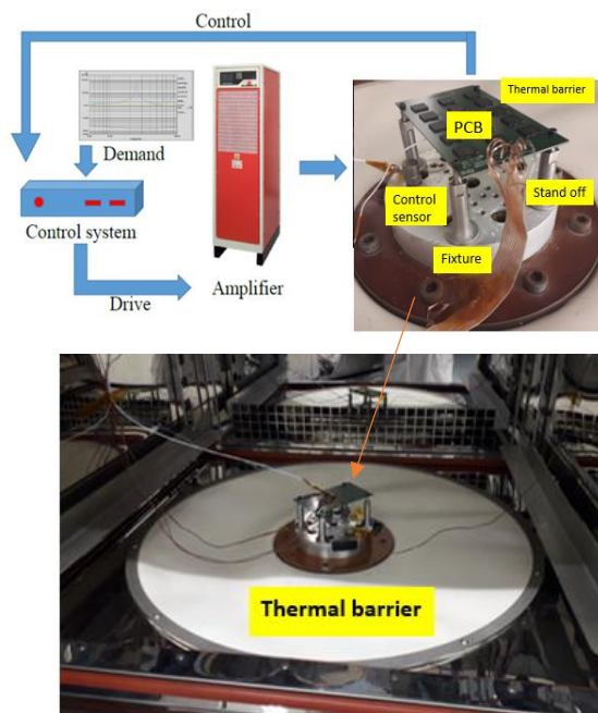
Fig. 4: Board Level Vibration Test Setup with thermal barrier at the bottom of the chamber
