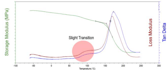
Fig. 12: Dynamic Mechanical Analysis (DMA) of Test Board
