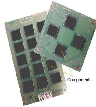
Fig. 3: Test Boards: Rectangular and Square PCBs
