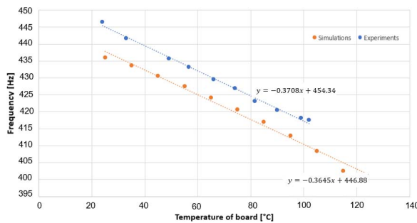
Fig. 19: Comparison of Simulation Results vs. Experimental Results
