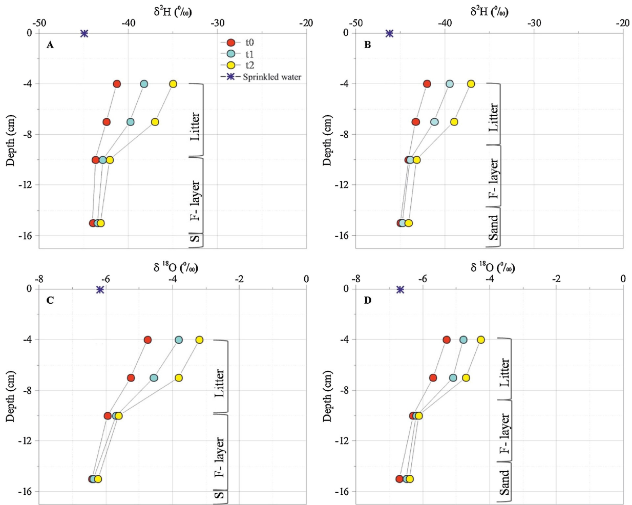
Fig. 7. Isotope depth profile in litter and fermentation layer at different days from the simulated rain (t0 = day of the sprinkling, t1 = 1 day after sprinkling and t2 = 2 days after sprinkling) in unburned (A, C) and burned (B, D) areas in P. pinaster (TAV) plantation. F-layer = Fermentation layer; S = Sand.
