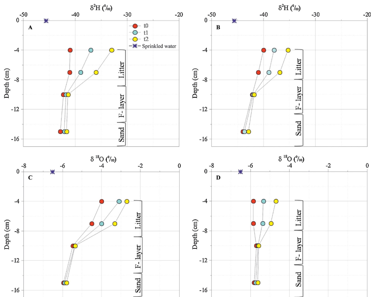
Fig. 5. Isotope depth profile in litter and fermentation layer at different days from the simulated rain ( t_0 = day of the sprinkling, t_1 = 1 day after sprinkling and t_2 = 2 days after sprinkling) in unburned (A, C) and burned (B, D) areas in P. pinea (CVR) plantation. F-layer = Fermentation layer.
