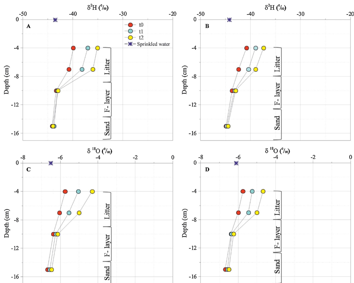
Fig. 6. Isotope depth profile in litter and fermentation layer at different days from the simulated rain ( t_0 = day of the sprinkling, t_1 = 1 day after sprinkling and t_2 = 2 days after sprinkling) in unburned (A, C) and burned (B, D) areas in P. halepensis (CNP) plantation. F-layer = Fermentation layer.
