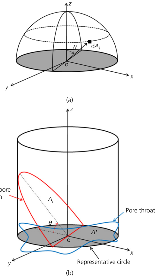
Figure 7. Model for a local throat on the basis of its representative circle (b) and associated unit sphere (a) onto which infinitely small elements of the random section areas are collected. Projection of dA_i yields a \cos term, whereas relative frequency is governed by a sine term (dashed line in (a))
