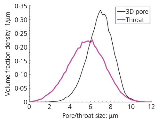
Figure 5. Volume-based 3D pore size distribution function and 2D throat size distribution function obtained by SVM (specimen W40F300 (i.e. w/c = 0.4 ; Blaine fineness = 300 \text{ m}^2/\text{kg} ))
