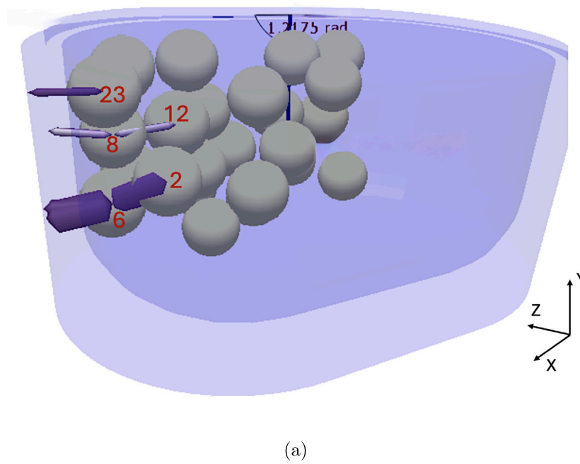
Fig. 1. (a) Schematic of jar movement ( A = 1.7 cm, n = 300 rpm) (b) 3D model of the milling jar [4].
