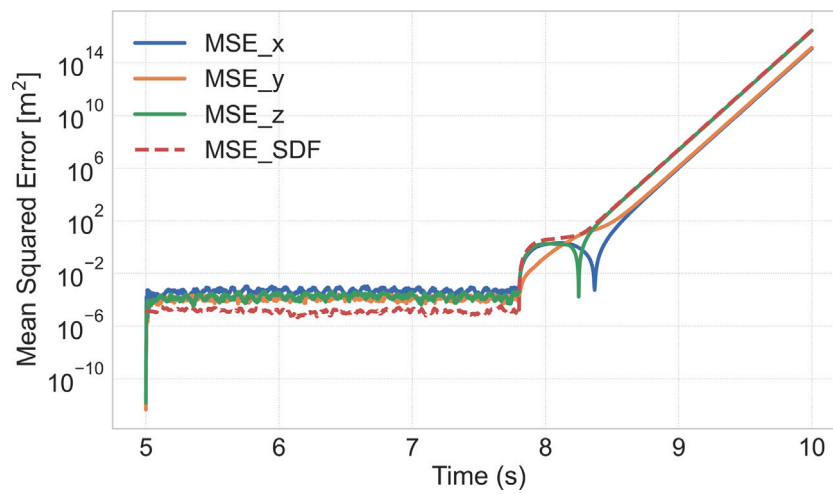
Fig. A.4. MSE loss history for interaction layer size = 4.
