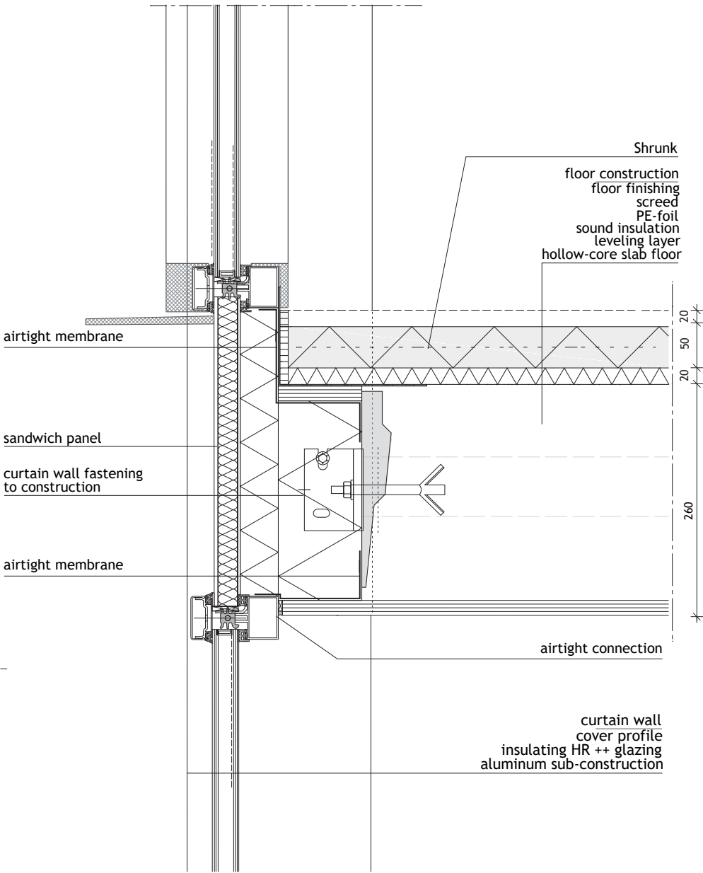
DETAIL 1:5
