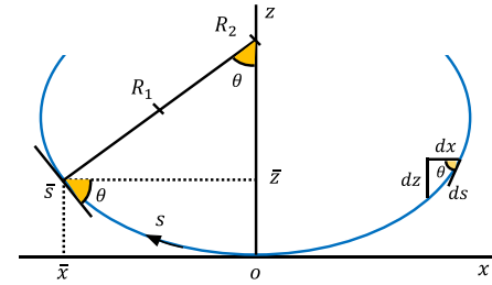
Fig. 3. Schematic of an axisymmetric drop, modified after Li et al. (1992).
