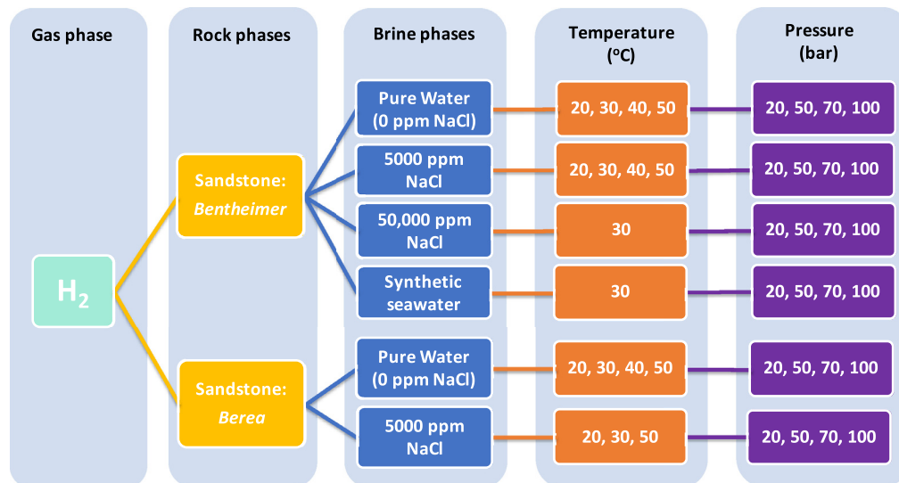
Fig. 5. Experimental conditions for hydrogen tests.
