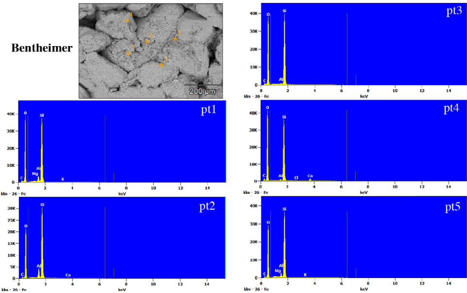
Fig. 10. SEM data of Bentheimer sandstone.
