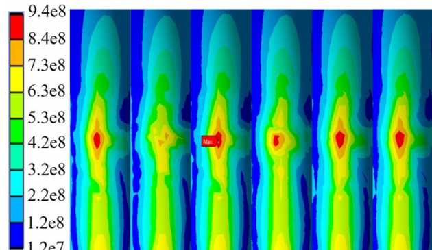
Fig. 7. The contact stress between ball key and ball seat
