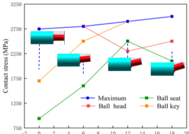
Fig. 15. Contact stress variation of flexible joints with different deflection angles
