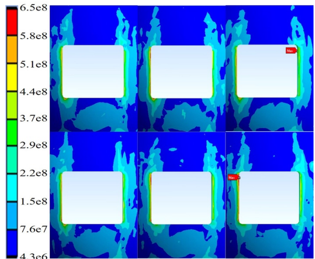
Fig. 13. The contact stress between ball seat and ball cage
