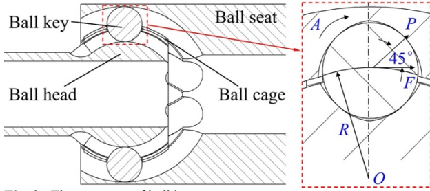
Fig. 2. The structure of ball key
