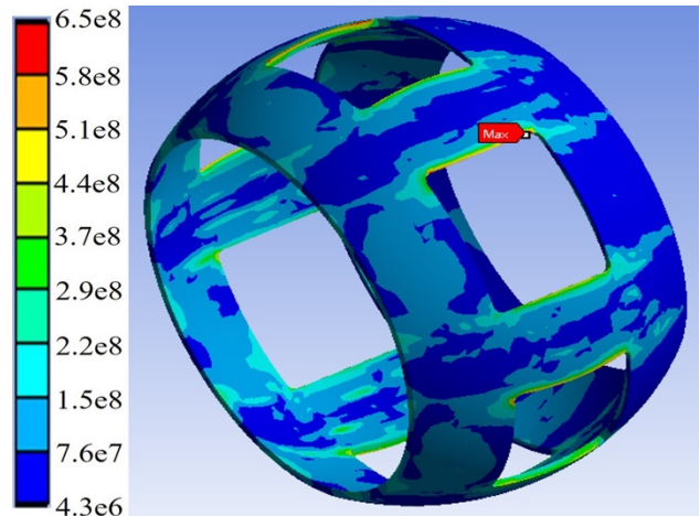
Fig. 12. The contact stress of ball cage
