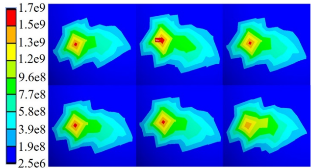
Fig. 11. The contact stress between ball head and ball key
