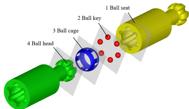
Fig. 1. Structure diagram of ball cage flexible joint
