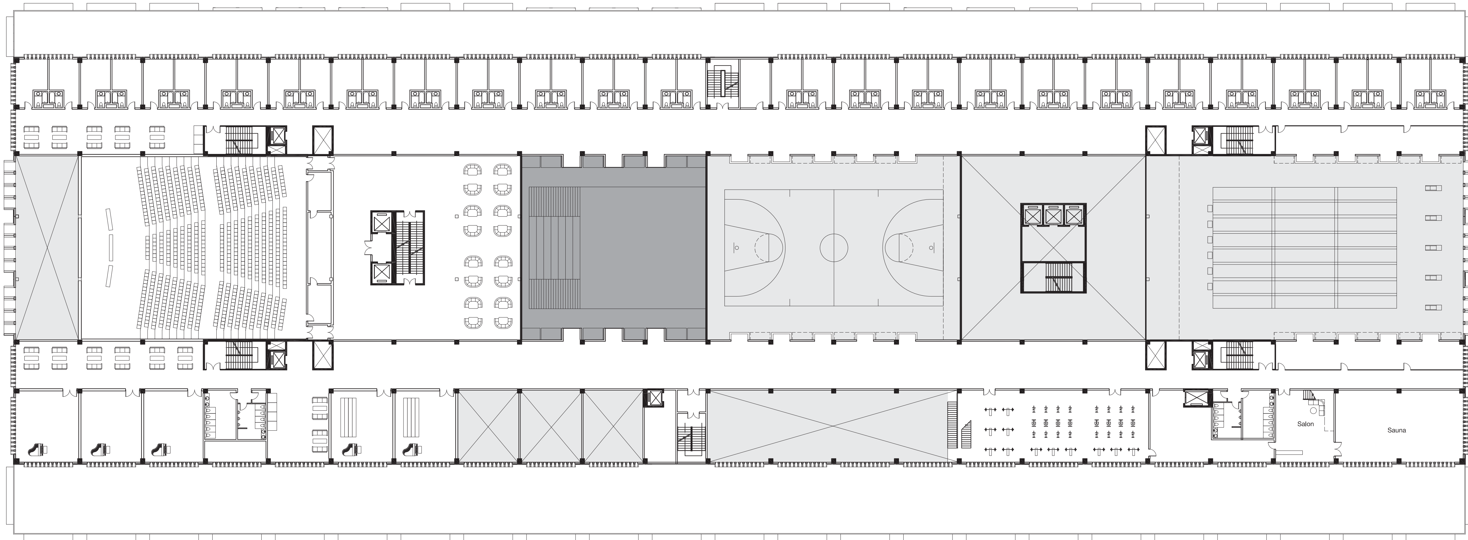
5TH FLOOR PLAN 1:300
