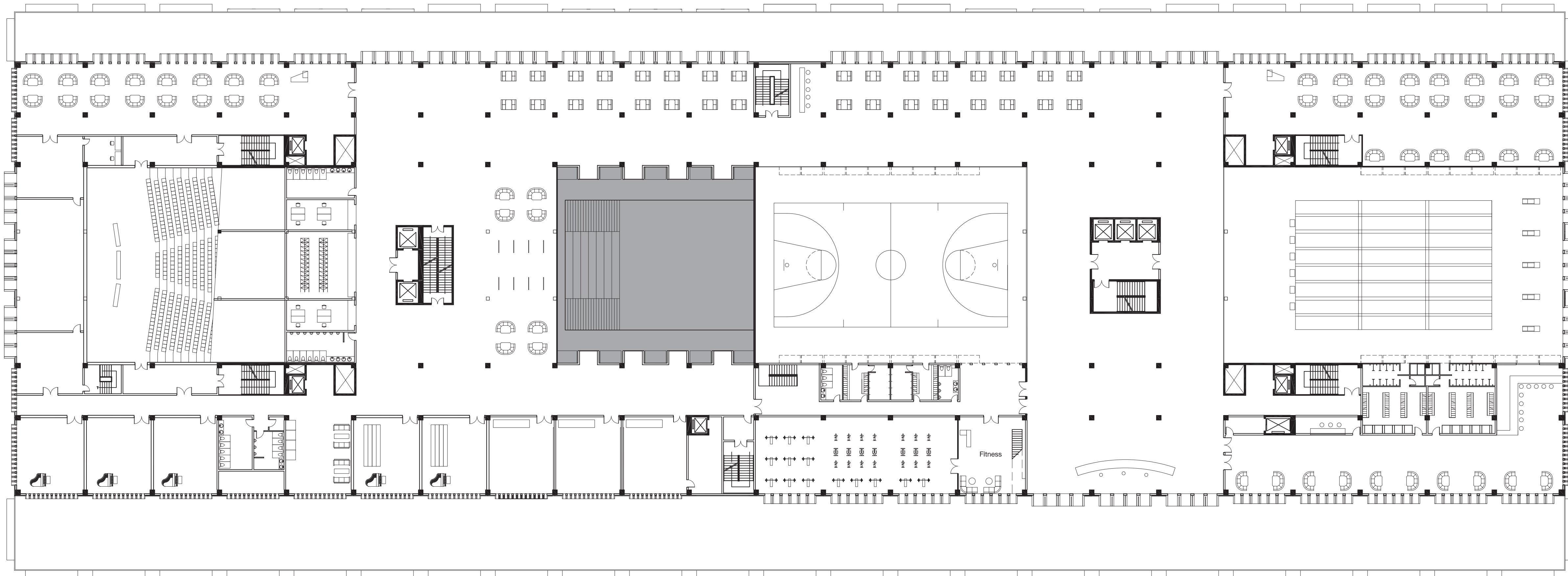
4TH FLOOR PLAN 1:300
