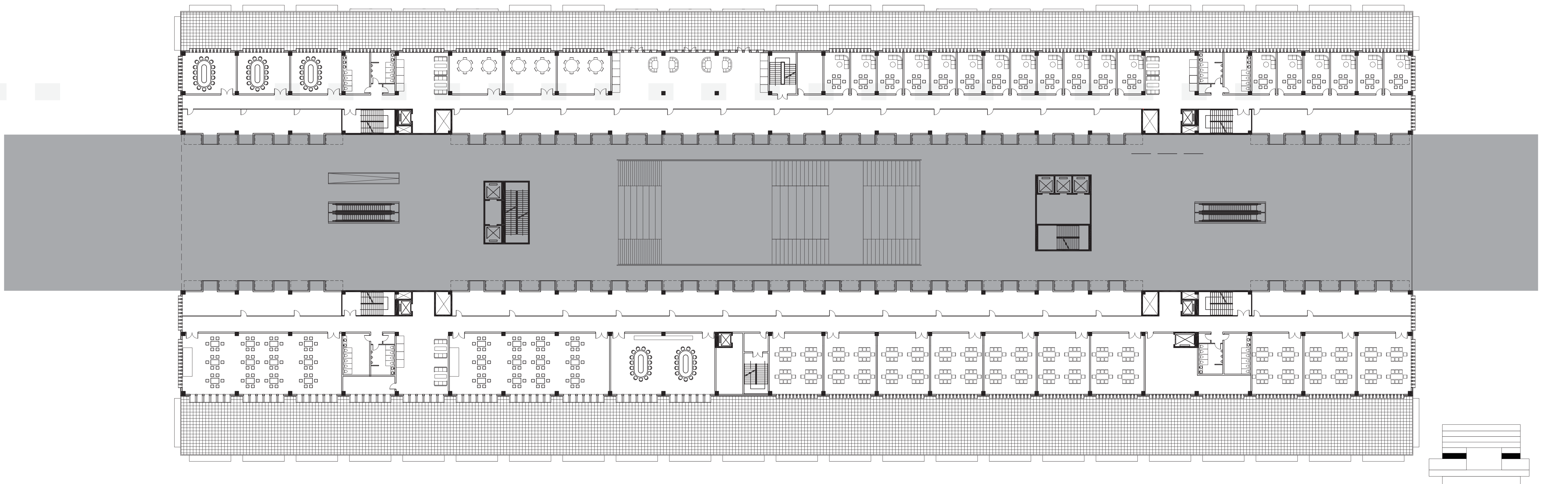
1ST FLOOR PLAN 1:300
