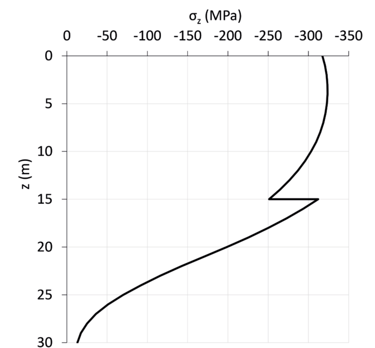
Fig. 3 Depth variation of the maximum vertical normal stress ( \sigma_z ) in the pile.
