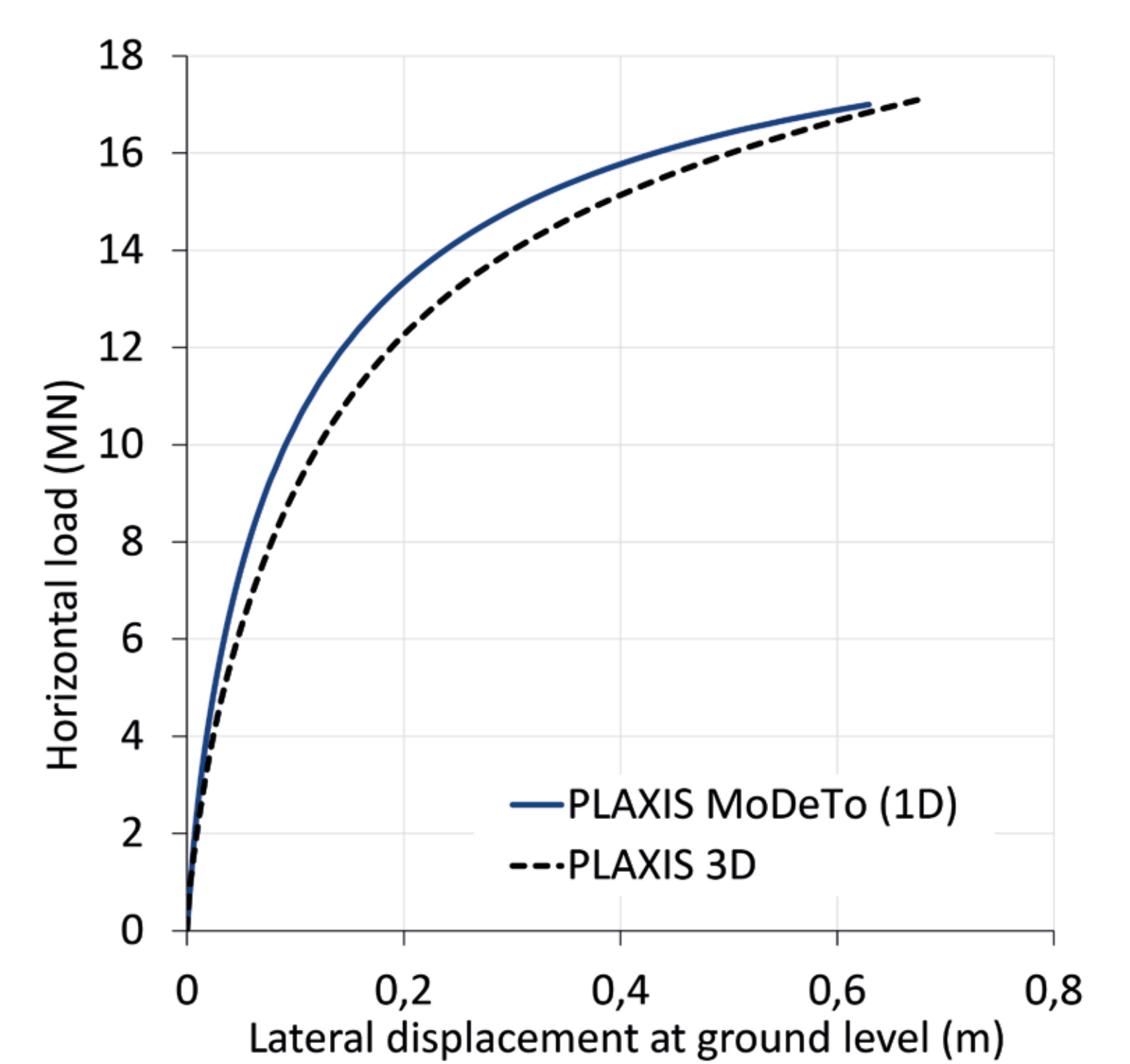
Fig. 5 Comparison between the 1D model and a 3D FE model for the final design.
