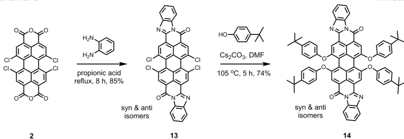
Scheme 4. New direct approach to synthesize 1,6,7,12-tetraphenoxyperylene bisbenzimidazole 14 .
