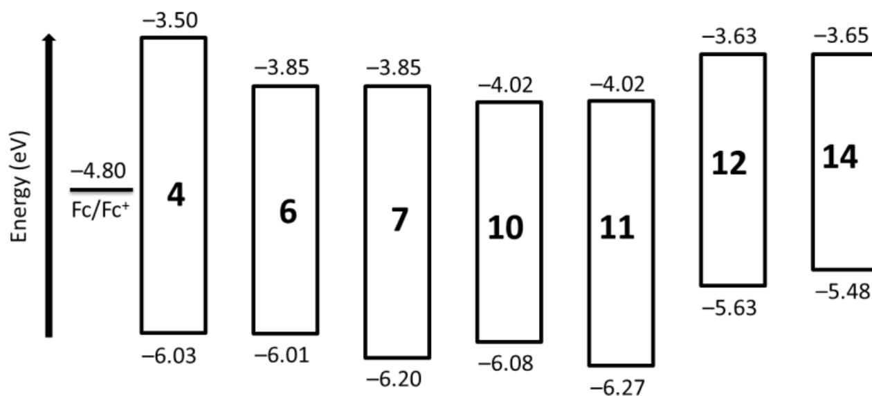
Figure 4. The HOMO and LUMO levels of synthesized perylene derivatives against vacuum.
