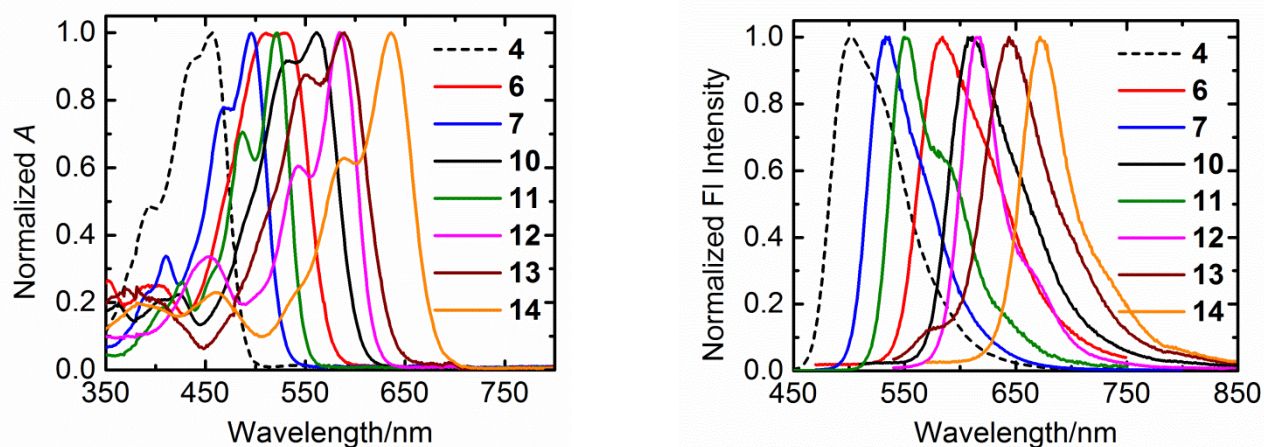
Figure 3. The normalized UV/Vis absorption (Left) and emission (Right) spectra of synthesized compounds in chloroform.
