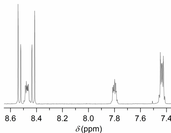
Figure 2. The ^1H NMR spectrum (aromatic region) of compound 14 .
