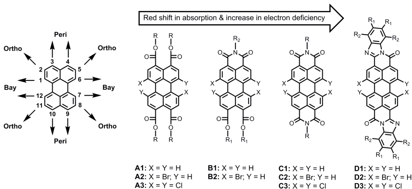
Figure 1. Previously prepared perylene-tetracarboxylic acid derivatives with tunable optical and electronic properties.
