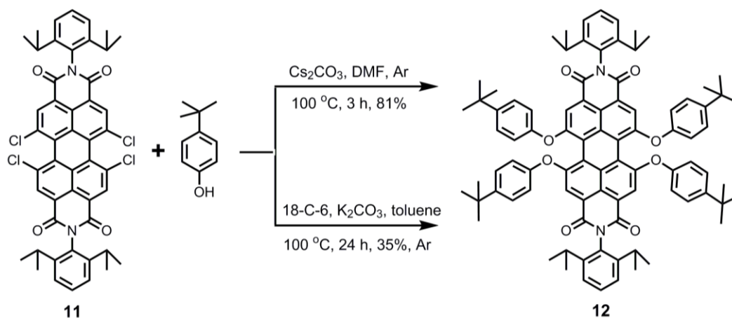
Scheme 3. Synthesis of 1,6,7,12-tetraphenoxy perylene bisimide 12 .
