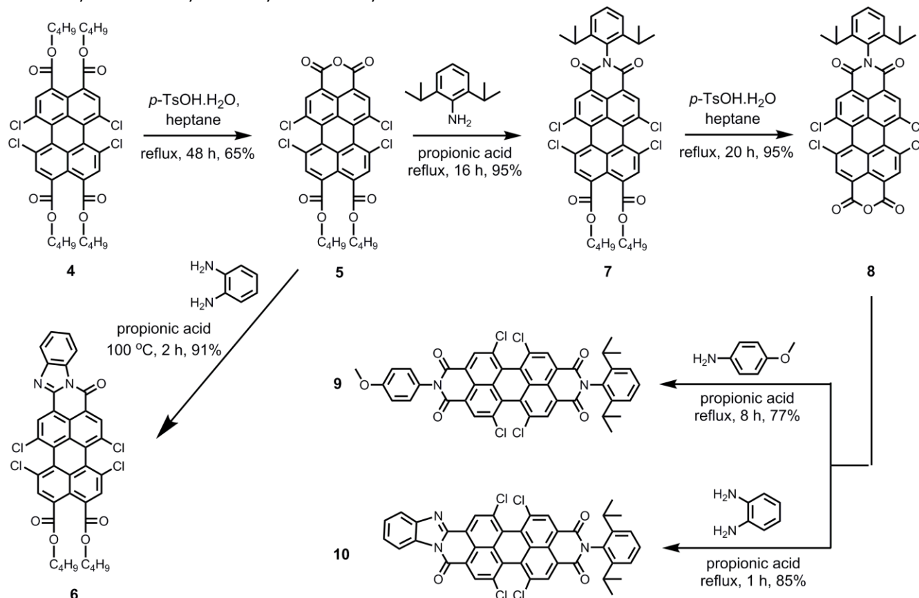
Scheme 2. Synthesis of novel 1,6,7,12-tetrachloro substituted perylene derivatives 5–10.
