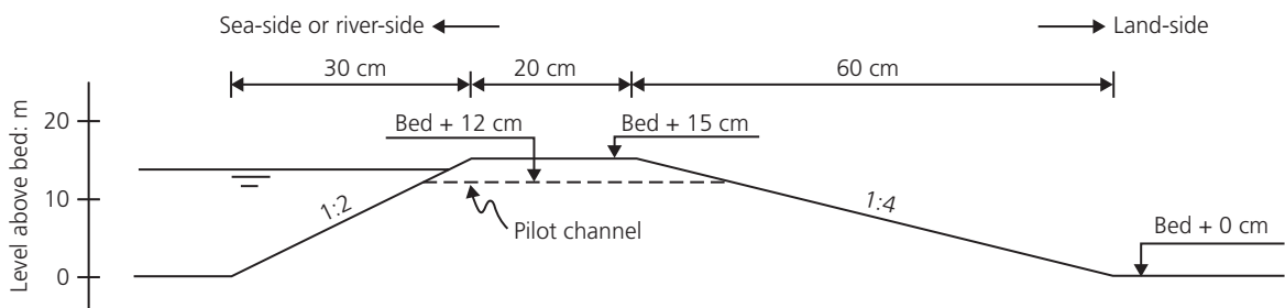
Figure 10. Cross-section of the Zwin'94 dike (Visser, 1998)
