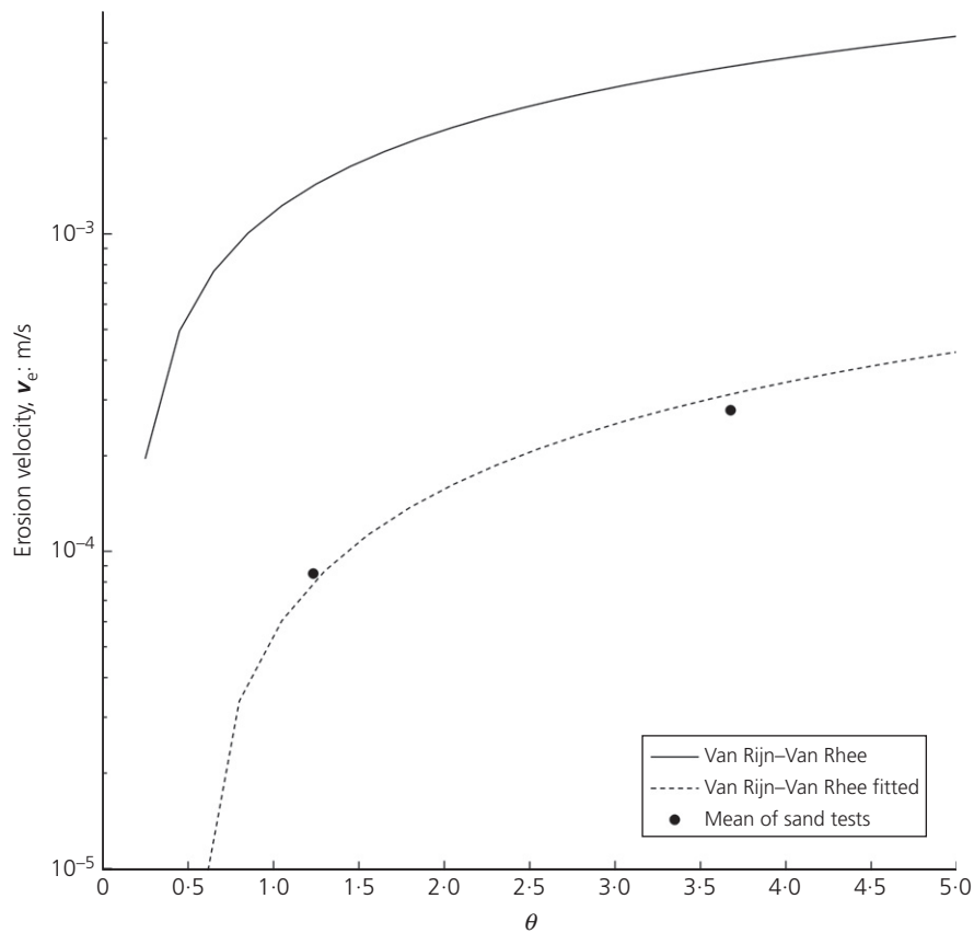
Figure 8. Comparison of test results with the Van Rijn–Van Rhee formula (Equation (10)) (for c_b=0 and k=k ) and fitted for the sand test (for c_b \approx 0.03 and k=k/20 )
