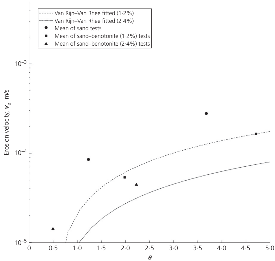
Figure 9. Fitting of the Van Rijn–Van Rhee formula (Equation (10)) (for c_b \approx 0.03 and k = k/20 ) to the results of the sand–bentonite tests (1.2% and 2.4%), by using permeability to the values measured
