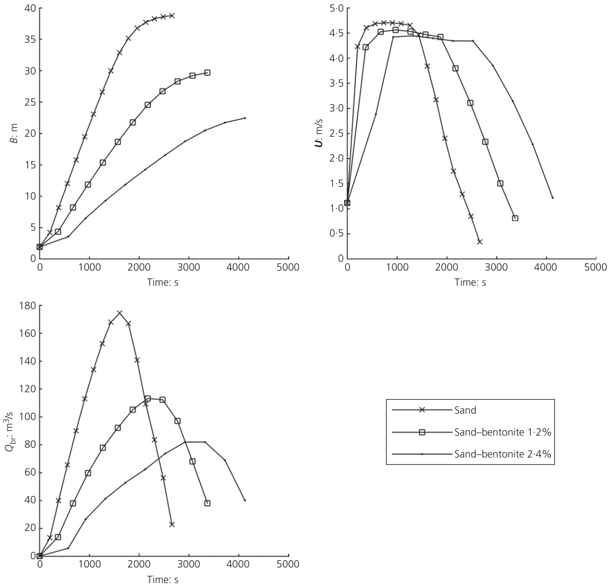
Figure 11. Comparison of results Bres model for the Zwin'94 dike for different added weight fractions of bentonite
