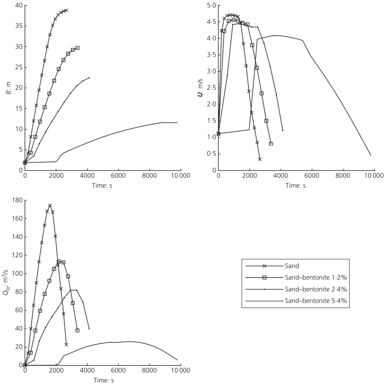
Figure 13. Comparison of Bres model results for the Zwin'94 dike for different added weight fractions of bentonite, including added bentonite percentage of 5.4%
