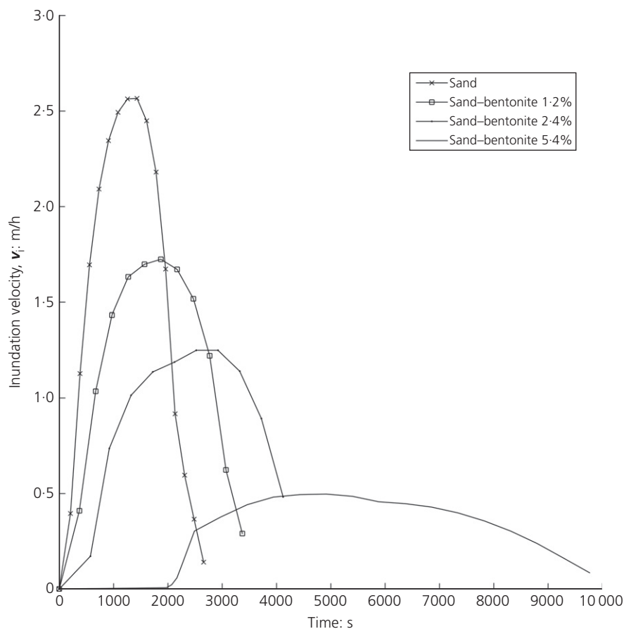
Figure 14. Comparison of inundation velocities in the Zwin'94 polder for different added weight fractions of bentonite, including necessary mixture (added bentonite percentage of 5.4%)
