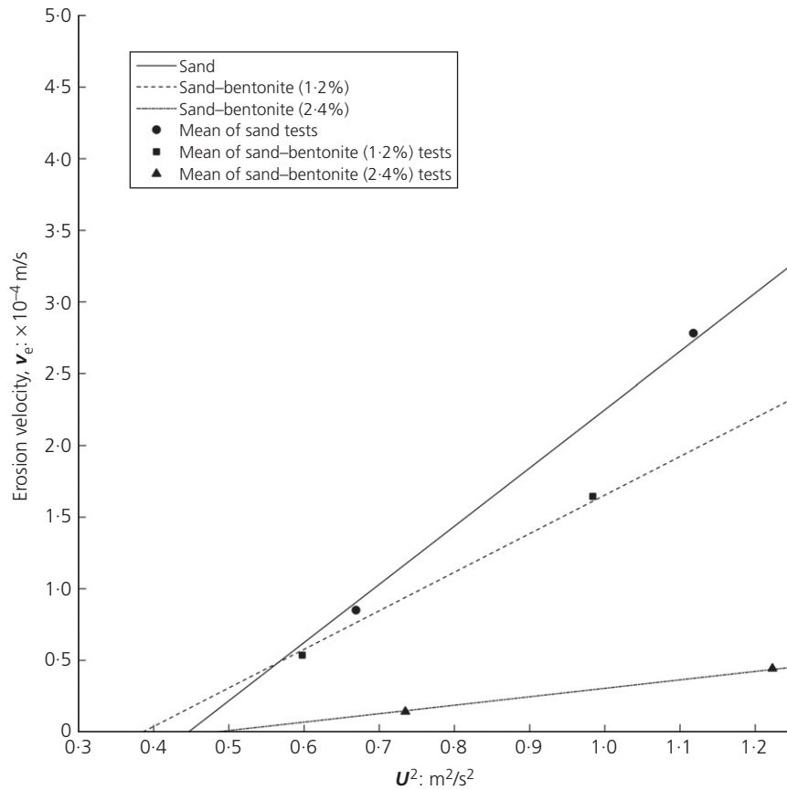
Figure 7. Crossing of U^2 -axis at v_e = 0 m/s of the linear regression lines (with mean results of experiments)
