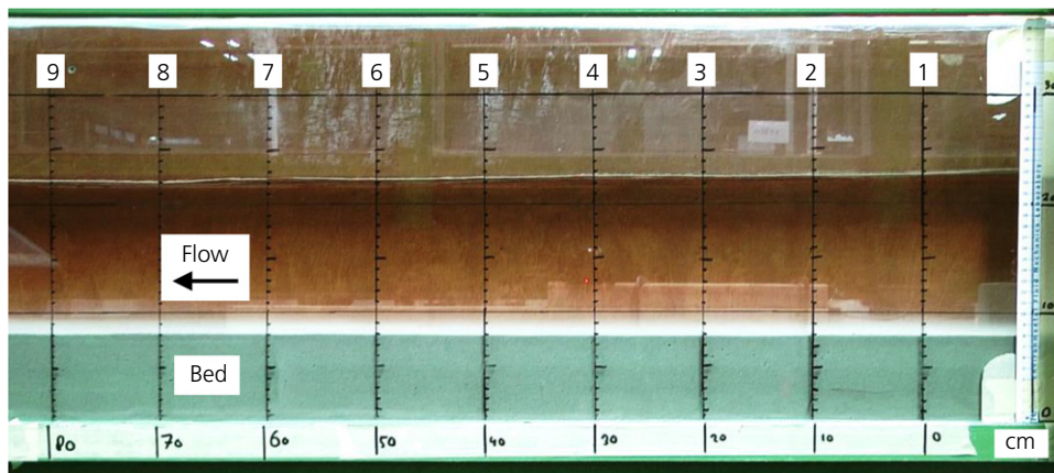
Figure 4. Measurement area and measurement locations (1–9)
