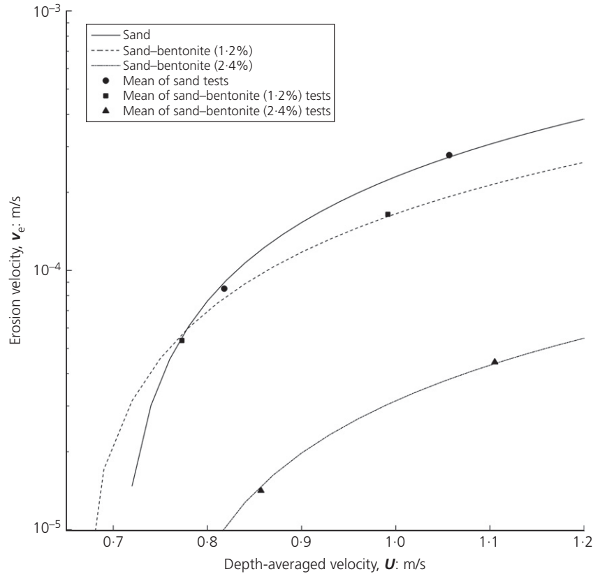
Figure 6. Linear regression lines and mean results of erosion experiment
