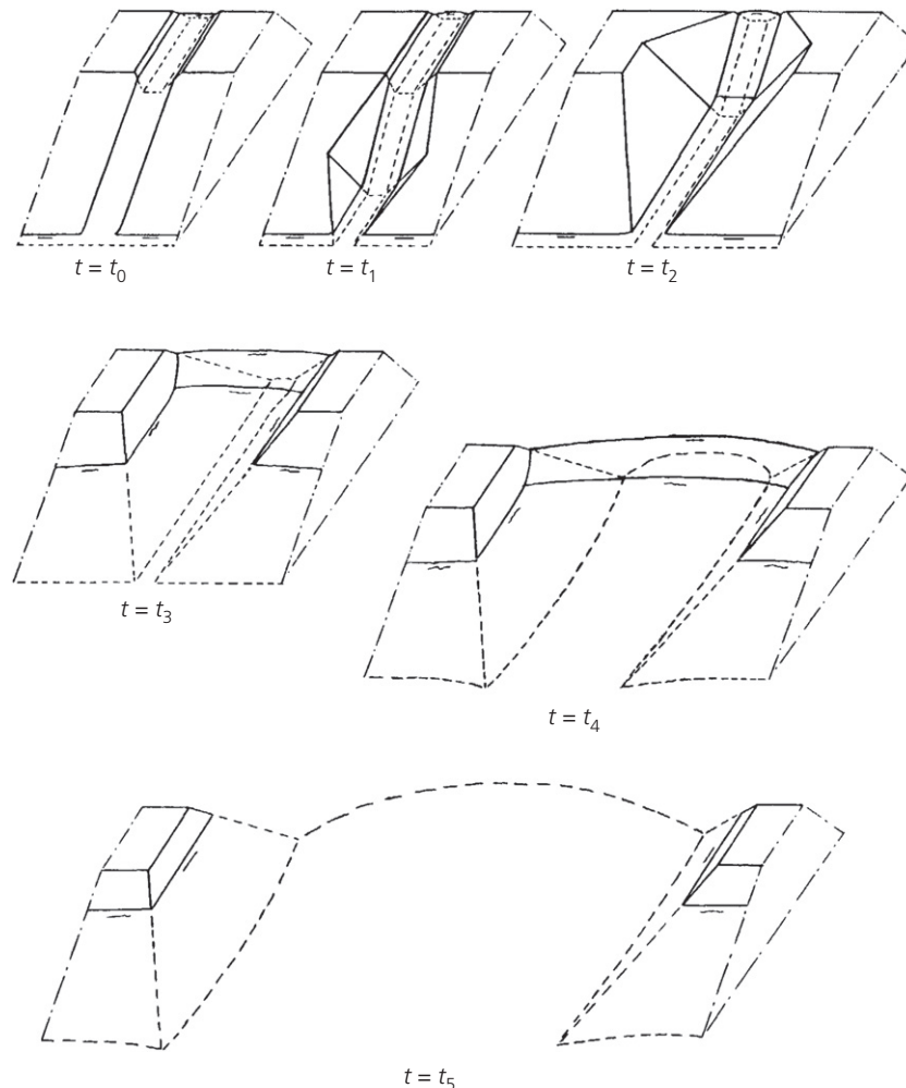
Figure 1. Schematic overview of the breaching process of a sand dike (Visser, 1998)
