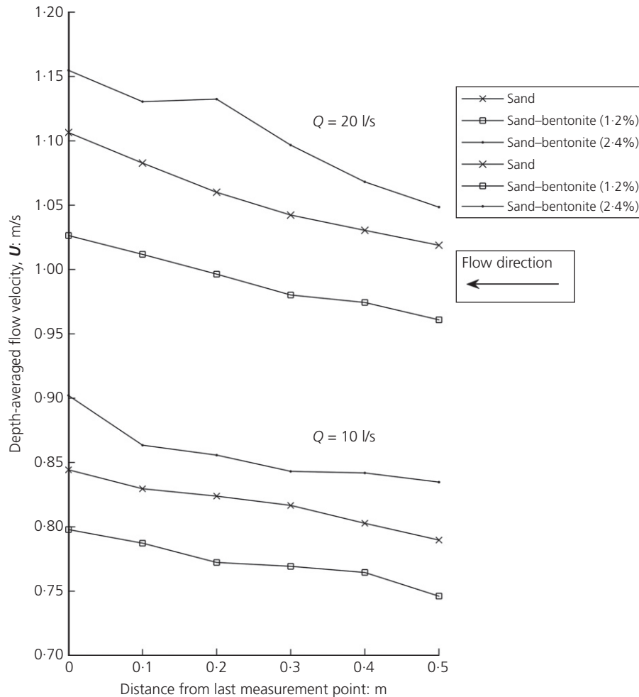
Figure 5. Depth-averaged flow velocities per test (measurement locations 4=0.5 m to 9=0 m)
