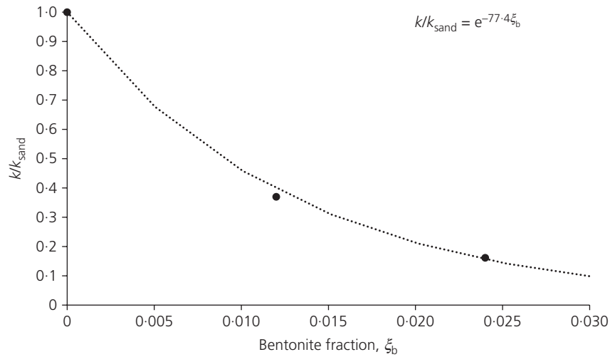
Figure 3. Reduction of permeability as a function of weight fraction of added bentonite
