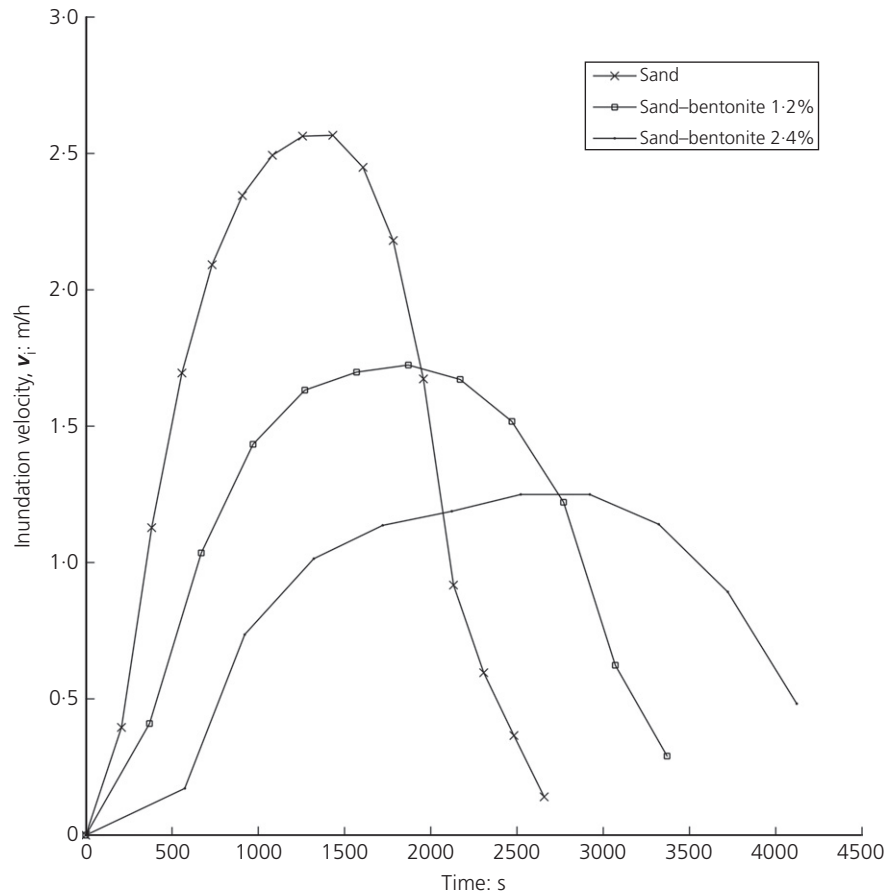
Figure 12. Comparison of inundation velocities in the Zwin'94 polder for different added weight fractions of bentonite
