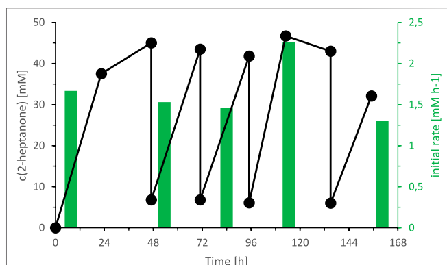
FIGURE 10 | Effect of replacing the organic layer on the SyADH catalysed oxidation of rac -heptan-2-ol in a biphasic reaction system. Reaction conditions: [rac\text{-heptan-2-ol}]_{org} = 50 mM, [ethyl\ acetoacetate]_{org} = 50 mM (1 equiv.), the organic phase was replaced at t = 47, 72, 96 and 135 h, [NADP^+]_{aq} = 1 mM, [E. coli\ C43(DE3)\ pET24b\text{-}syadh]_{aq} = 5\ mg \times mL^{-1} , [KPi, pH\ 7] = 1 M (10% v/v), [n\text{-heptane}] = 90\% v/v, total volume: 500 \mu L , T = 30^\circ C , 600 rpm.
