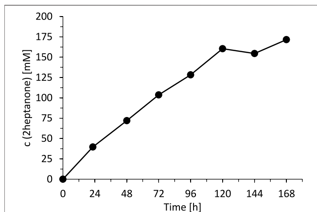
FIGURE 9 | Fed-batch transformation of rac -heptan-2-ol. Reaction conditions: [rac\text{-heptan-2-ol}]_{org} = [ethyl\ acetoacetate]_{org} : added (50 mM each) at t = 0, 22.5, 48, 72, 96 and 120 h, [NADP^+]_{aq} = 1 mM, [E. coli\ C43(DE3)\ pET24b\text{-}syadh]_{aq} = 5\ mg \times mL^{-1} , [KPi, pH\ 7] = 1 M (10% v/v), [n\text{-heptane}] = 90\% v/v, total volume: 500 \mu L , T = 30^\circ C , 600 rpm.
