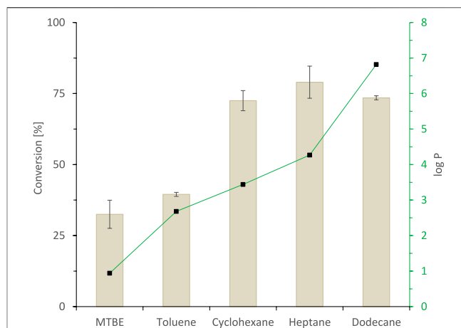
FIGURE 4 | The effect of hydrophobicity of organic solvent (expressed as log p values (■)) on the activity of SyADH-catalysed oxidation of rac -heptan-2-ol in biphasic reaction systems. Reaction conditions: [ rac -heptan-2-ol] organic phase = 50 mM, [ethyl acetoacetate] organic phase = 100 mM (2 equiv.), [NADP + ] aq = 1 mM, [ E. coli C43 (DE3) pET24b- syadh ] aq = 10 mg × mL -1 , [KPi, pH 7] = 1 M (10% v/v), [organic solvent] = 90% v/v, total volume: 500 μL, T = 30°C, reaction time: 24 h, 600 rpm. Data are expressed as the mean ± SD of the two independent experiments performed in technical duplicates.
