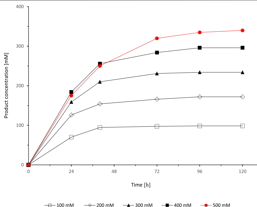
FIGURE 6 | Effect of different substrate concentrations on the SyADH catalysed oxidation of rac -heptan-2-ol in a biphasic reaction system. Reaction conditions: [rac\text{-heptan-2-ol}]_{org} = 100\text{--}500\text{ mM} , [ethyl\ acetoacetate]_{org} = 100\text{--}500\text{ mM} (1 equiv.), [NADP^+]_{aq} = 1\text{ mM} , [E. coli\ C43(DE3)\ pET24b\text{-}syadh]_{aq} = 5\text{ mg}\times\text{mL}^{-1} , [KPi, pH\ 7] = 1\text{ M} (10% v/v), [heptane] = 90\% v/v, total volume: 500\text{ }\mu\text{L} , T = 30^\circ\text{C} , 600 rpm.
