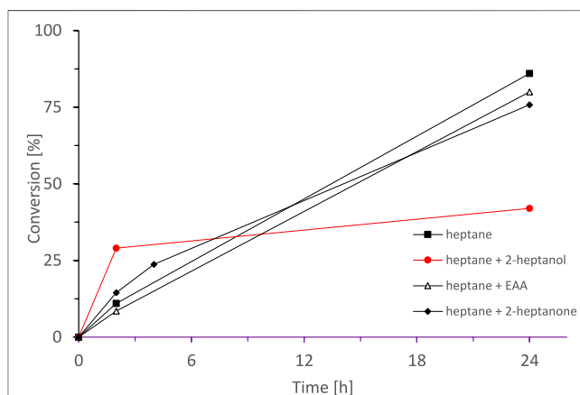
FIGURE 8 | Effect of pre-incubation of the SyADH whole cell-biocatalyst in the presence of different reagents on its catalytic activity. Lyophilised cells were incubated for 72 h in (\blacksquare) n -heptane, (\bullet) rac -heptan-2-ol (in n -heptane), (\Delta) ethyl acetoacetate (in n -heptane) and (\blacklozenge) 2-heptanone (in n -heptane), then the remaining components were added. Reaction conditions: [rac\text{-heptan-2-ol}] = 100\text{ mM} , [Ethyl\ acetoacetate] = 100\text{ mM} (1 equiv.), [NADP^+] = 0.5\text{ mM} , [E. coli\ C43(DE3)\ pET24b\text{-}syadh] = 5\text{ mg}\times\text{mL}^{-1} , [KPi, pH\ 7] = 1\text{ M} (10% v/v), [n\text{-heptane}] = 90\% v/v, total volume: 10 ml, T = 30^\circ\text{C} , 230 rpm.
