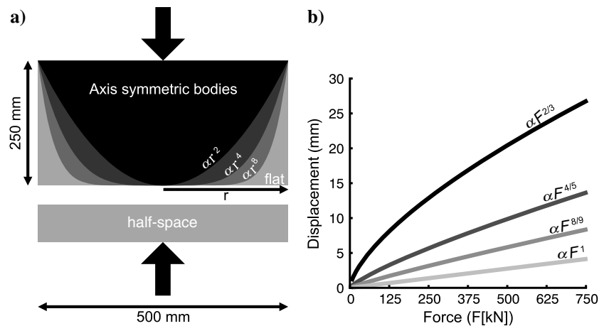
Figure 2. The 3D axis symmetric bodies. (a) Different gray scales and (b) their force-displacement relation when pressed onto a half-space of the same material. The black arrows indicate the direction of the force and displacement. Values for parameters: shear modulus: 200 MPa; Poisson’s ratio of 0.45.
