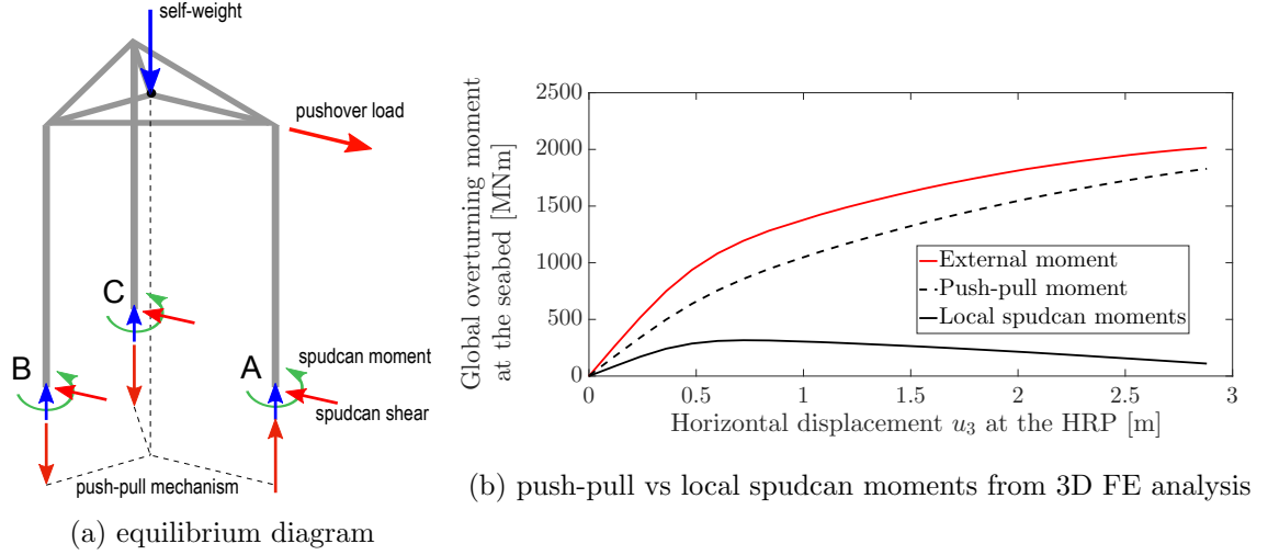
Figure 11: Evolution of moment-resisting mechanisms during symmetric pushover.
