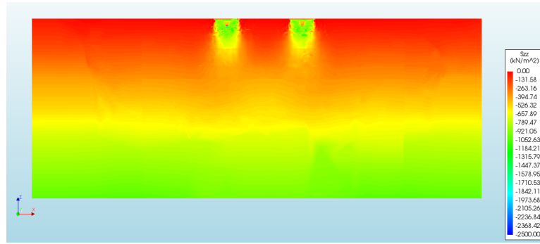
(b) vertical soil stress contours – after preloading
