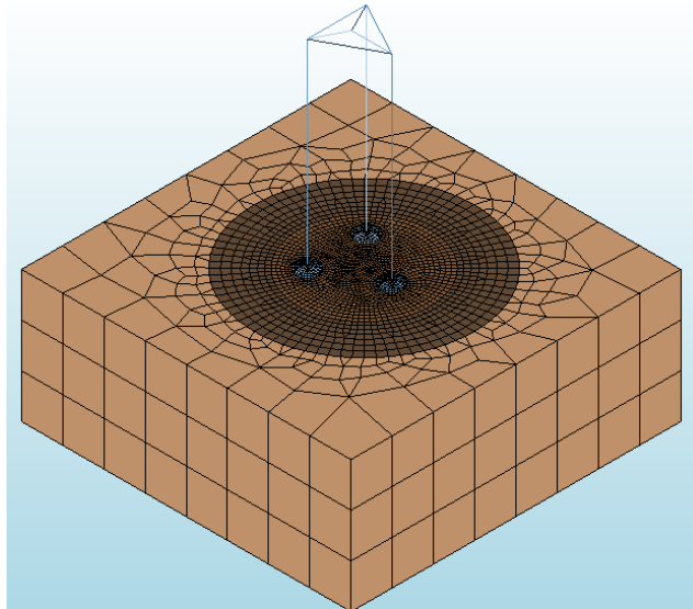
Figure 5: FE mesh of the jack-up-spudcans-soil 3D model.
