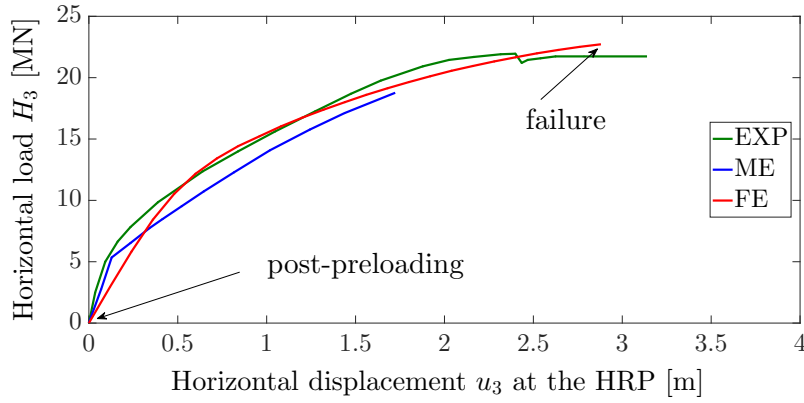
(a) horizontal force-displacement response at the hull – comparison among EXP, ME and FE results
