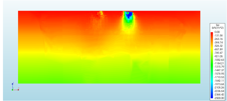
(c) vertical soil stress contours – at failure
