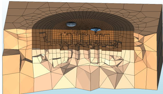
(a) 3D model domain partition
