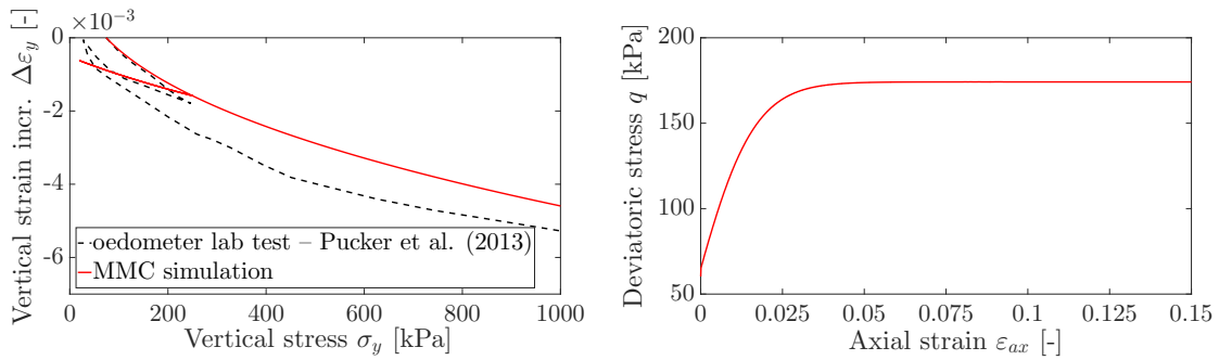
(a) oedometer test – laboratory test data from Pucker et al. (2013) (b) triaxial test – MMC simulation based on data from Pucker et al. (2013) and Cheong (2002)
