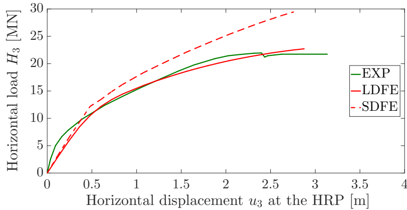
Figure 8: Influence of geometrical non-linearity on the jack-up response to symmetric pushover.
