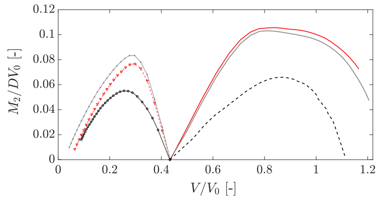
(b) moment-vertical ( M_2/DV_0 - V/V_0 )
