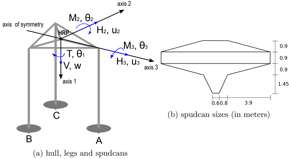
Figure 3: Structural components of the jack-up FE model.
