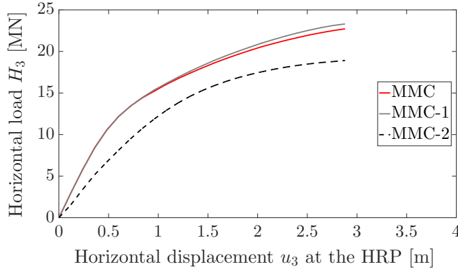
(c) comparison among global force-displacement responses at the hull.
