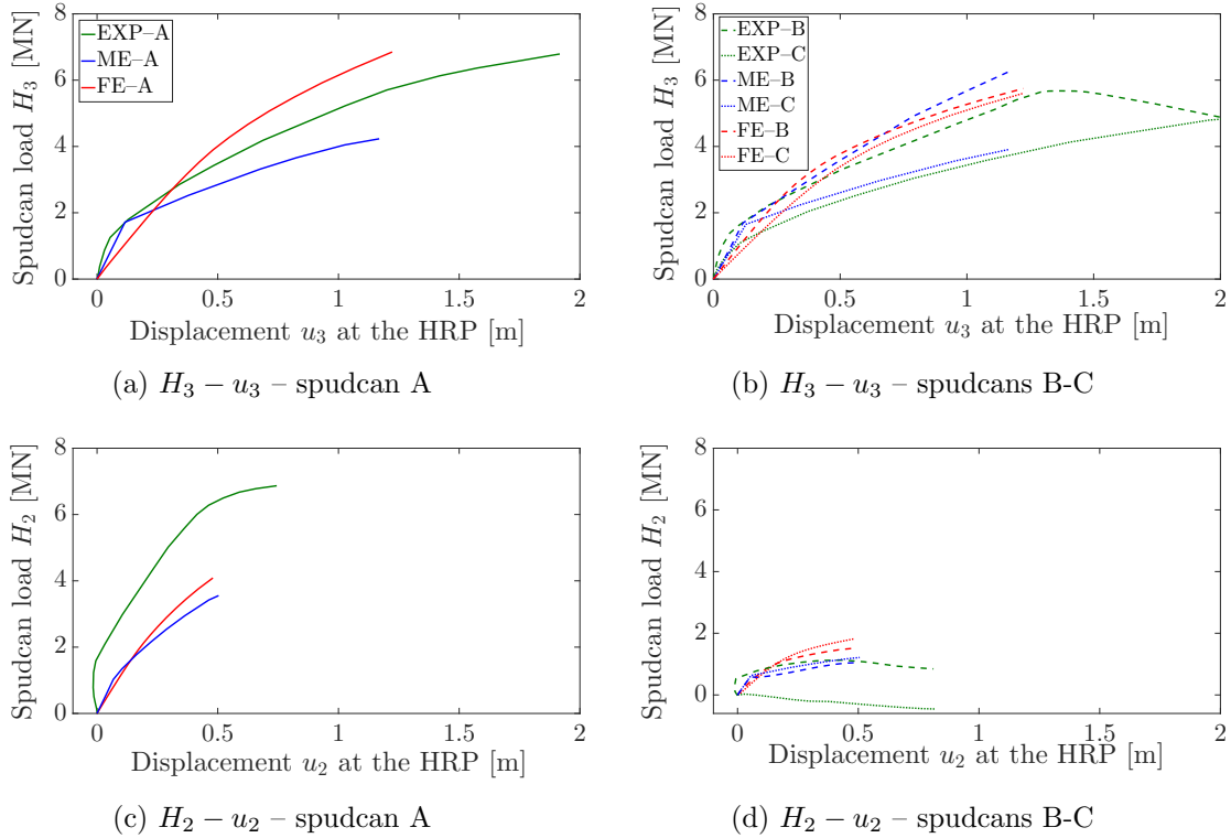
Figure 14: Spudcan force-displacement responses during misaligned pushover.
