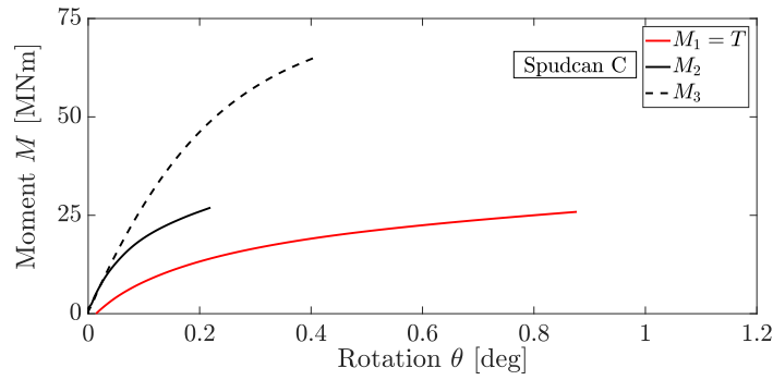
(b) moment-rotation responses ( M_1/DV_0 - \theta_1 , M_2/DV_0 - \theta_2 , M_3/DV_0 - \theta_3 ) at spudcan C
