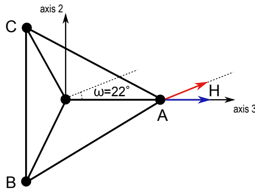
Figure 6: Orientation of the lateral loads in validation pushover analyses.
