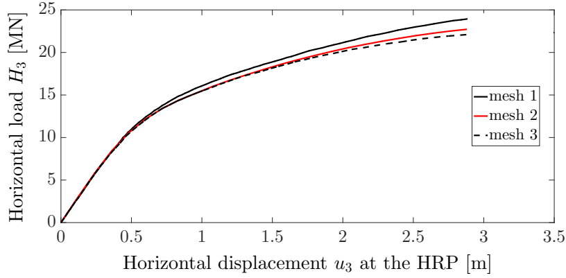
Figure 21: Jack-up performance under symmetric lateral pushover at varying FE discretisation – horizontal force-displacement response at the hull (Section 4.1).
