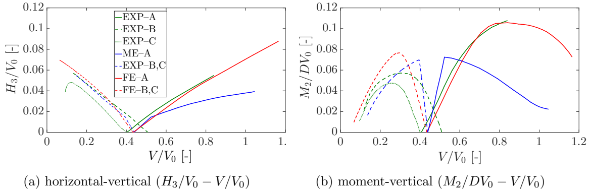
Figure 9: Spudcan load paths during symmetric pushover – Note : all experimental measurements on spudcan A terminated earlier than for spudcans B-C due exceeded bending gauge capacity (Bienen et al., 2009).
