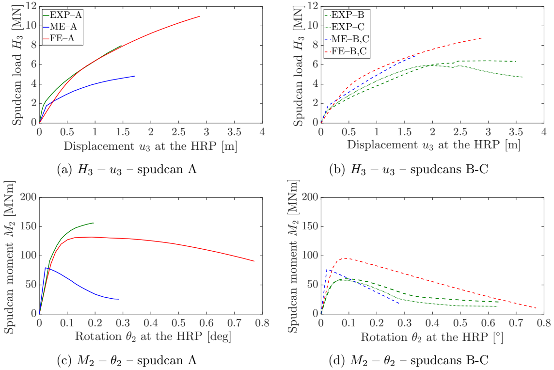
Figure 10: Spudcan force-displacement and moment-rotation responses during symmetric pushover – Note : all experimental measurements on spudcan A terminated earlier than for spudcans B-C due exceeded bending gauge capacity (Bienen et al., 2009).
