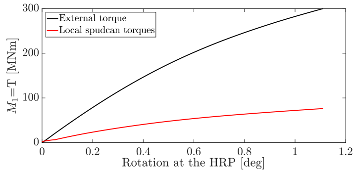
(a) torque-twist response at the hull and quota from the sum of single spudcan torques
