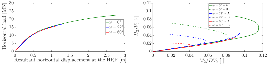
(a) horizontal force-displacement response at the hull (b) horizontal-moment spudcan load paths ( H_3/V_0 - M_2/DV_0 )
