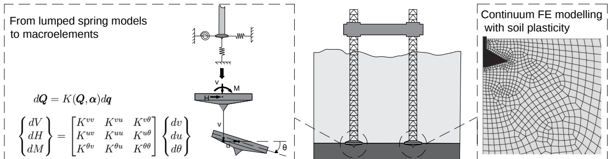
Figure 2: Lumped (left) vs continuum (right) modelling of soil-spudcan interaction.
