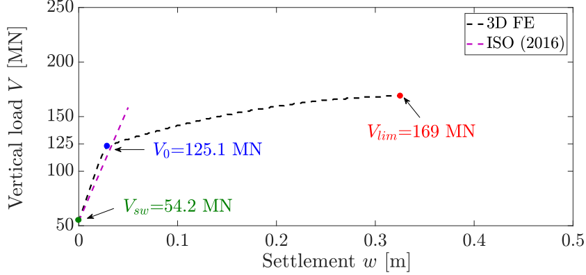
Figure 22: Simulated load-settlement response of a single spudcan.
