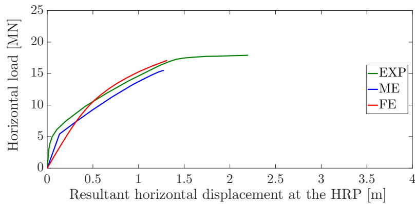
Figure 12: Jack-up response to misaligned pushover – comparison among EXP, ME and FE results.
