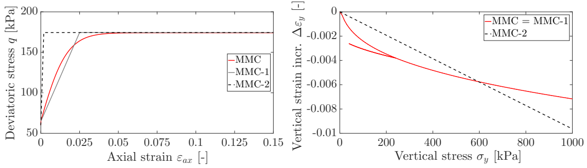
(a) comparison among triaxial performances (b) comparison among oedometric performances
