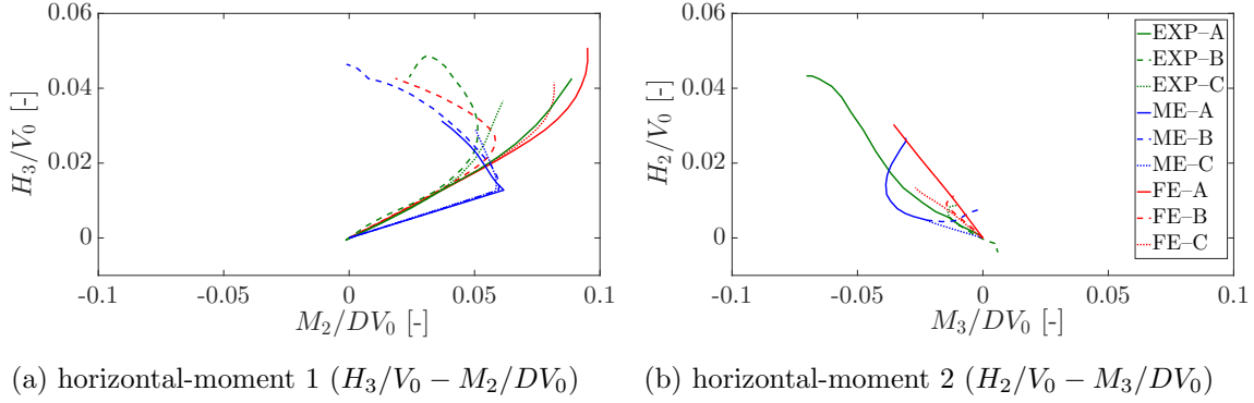
Figure 13: Spudcan load paths during misaligned pushover.
