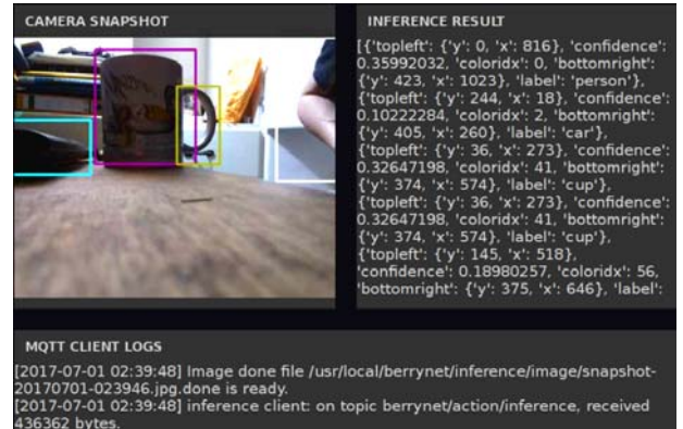
Fig. 4. Multiple-object detection via BerryNet [24]: 'person', 'cup'.
