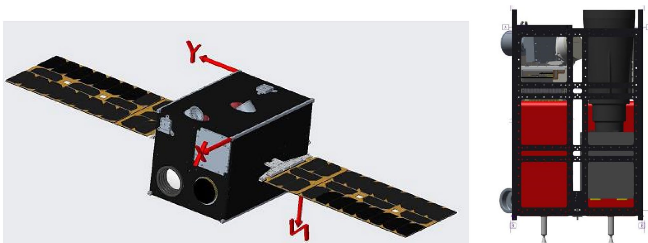
Fig. 10 Rendering (left) and internal view (right) of the LUMIO spacecraft (Phase A configuration) [21]
